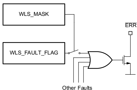
Figure 21. Weak-LED-Supply Fault-Report Topology
