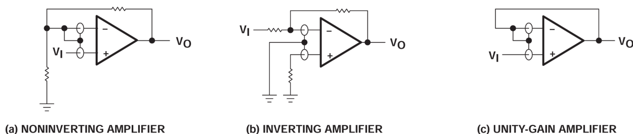
Figure 7-5. Guard-Ring Schemes
