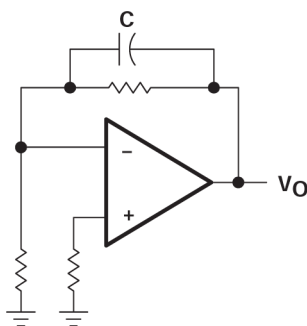
Figure 7-6. Compensation for Input Capacitance
