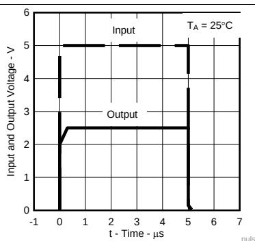
Figure 10. Pulse Response
