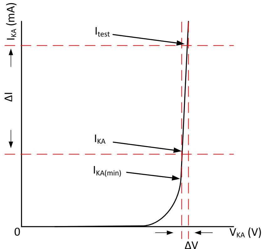
Figure 17. Dynamic Impedance
