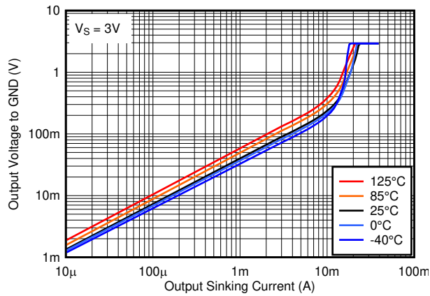
Figure 5-19. Output Low Voltage vs. Output Sinking Current at 3V
