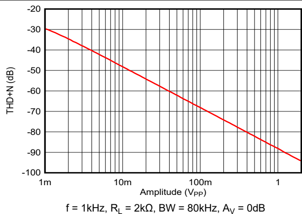
Figure 5-17. Total Harmonic Distortion + Noise vs Amplitude
