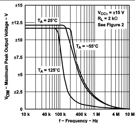
Figure 5-39. Maximum Peak Output Voltage vs Frequency
