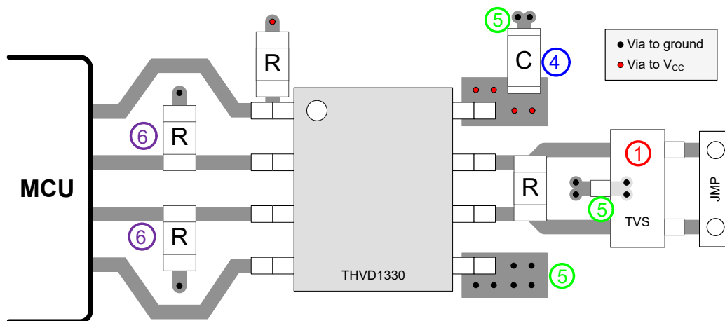
Figure 9-5. Layout Example
