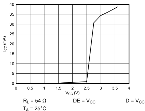
Figure 6-3. Supply Current vs Supply Voltage
