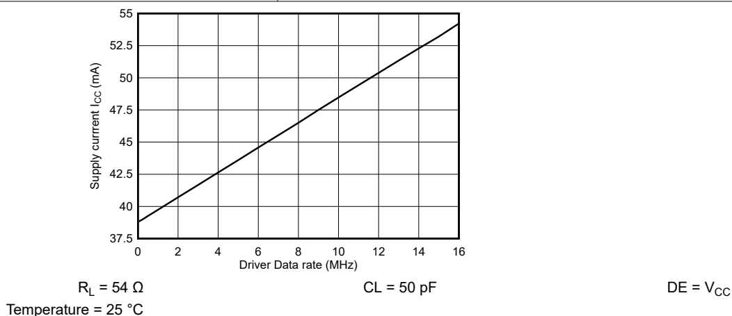
Figure 6-5. Supply Current vs Signal Rate
