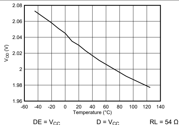
Figure 6-4. Driver output differential voltage vs Temperature
