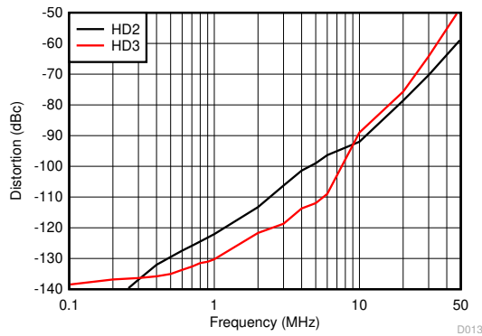
Figure 6-13. Harmonic Distortion Over Frequency
