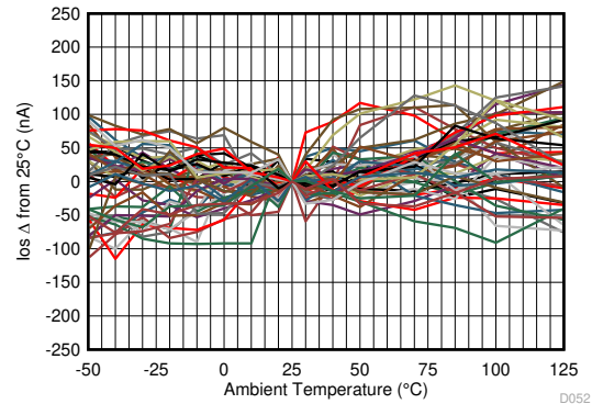
Figure 6-50. Input Offset Current
