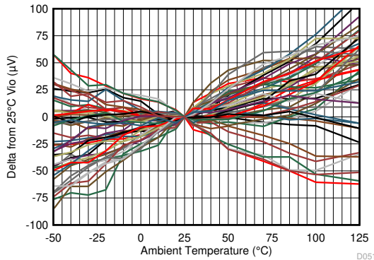
Figure 6-49. Input Offset Voltage
