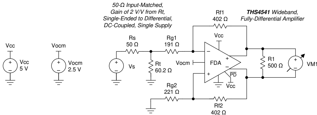
Figure 7-9. DC-Coupled Gain of 2 with R_f = 402\ \Omega and a Single-Ended to Differential Matched Input 50- \Omega Impedance
