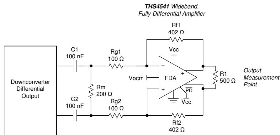
Figure 8-2. Example Down-Converting Mixer Delivering an AC-Coupled Differential Signal to the THS4541-Q1
