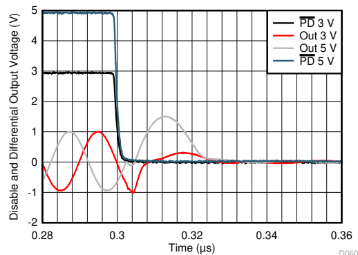
Figure 6-60. \overline{\text{PD}} Turn Off Waveform
