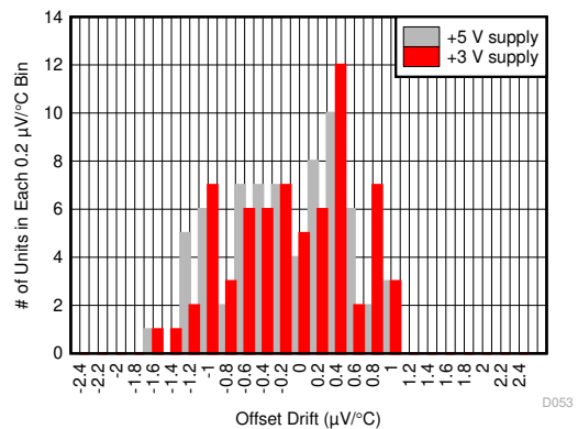
Figure 6-51. Input Offset Voltage Over Temperature
