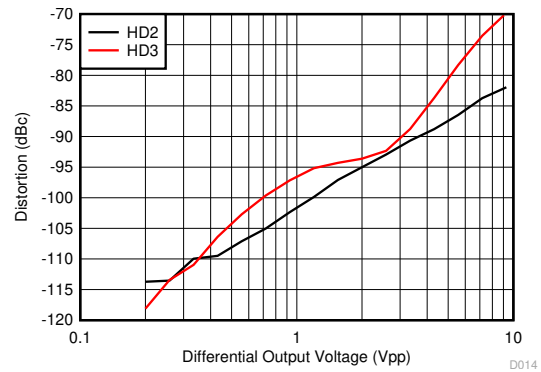
Figure 6-14. Harmonic Distortion vs Output Swing
