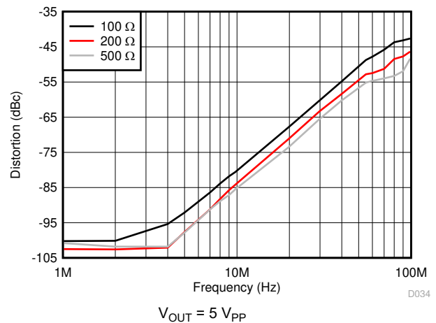
Figure 6-34. HD3 vs Load Resistance
