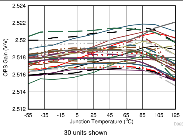
Figure 6-63. OPS Gain Over Temperature
