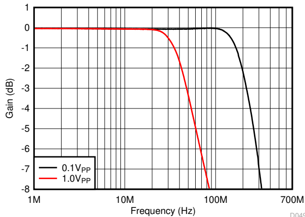
Figure 6-49. Frequency Response vs Output Voltage
