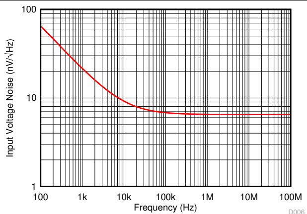
Figure 6-6. Input-Referred Differential Noise 25- \Omega source impedance on each D2S input
