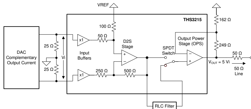
Gain = 5 V/V, Differential-to-Single-Ended Line Driver With Optional External Filter
