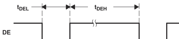
Figure 8-13. Minimum DE Low and Maximum DE High
