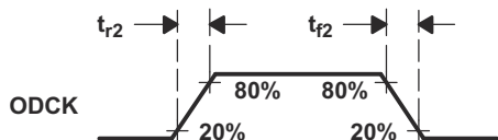
Figure 8-2. Rise and Fall Times of ODCK
