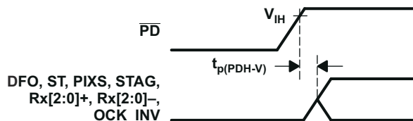
Figure 8-9. Delay From \overline{PD} Low to High Before Inputs Are Active
