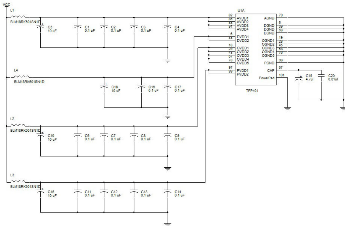
Figure 10-4. Power Supplies Decoupling Design
