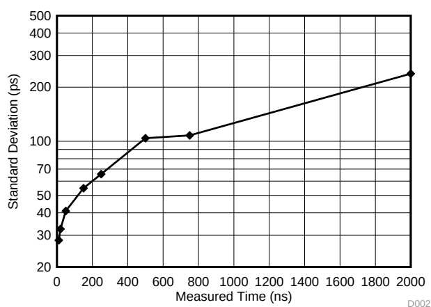
Figure 22. Measurement Mode 1 Standard Deviation vs Measured Time-of-Flight
