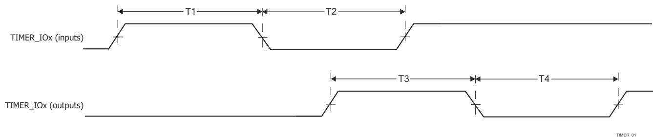
Figure 6-117. Timer Timing
