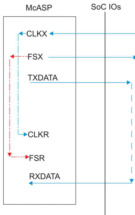
Figure 5-57. McASP1-8 CI-FO- – SYNC Mode
