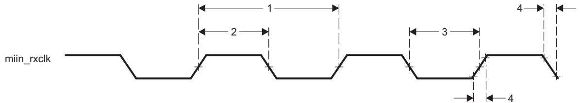
Figure 5-61. Clock Timing (GMAC Receive) - MII operation
