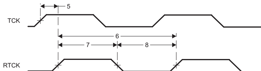
Figure 5-102. JTAG With RTCK Timing
