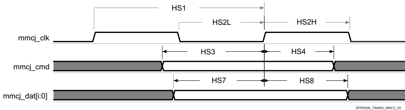
Figure 5-93. MMC/SD/SDIOj in - High Speed 3.3V Signaling - Receiver Mode
