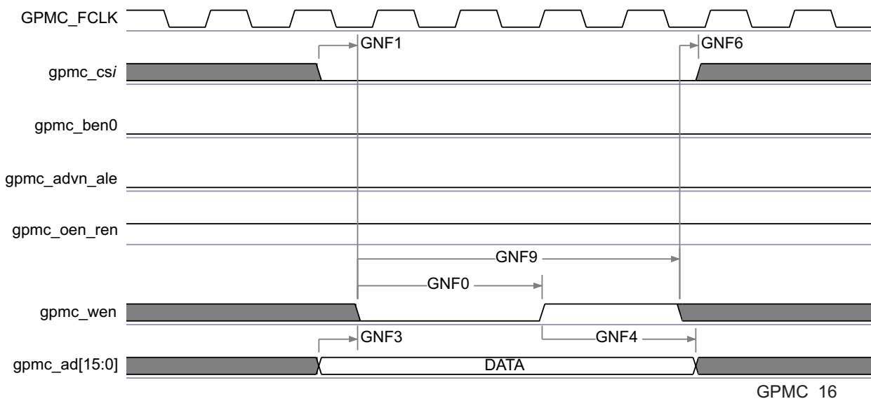
Figure 5-38. GPMC / NAND Flash - Data Write Cycle Timing (1)
