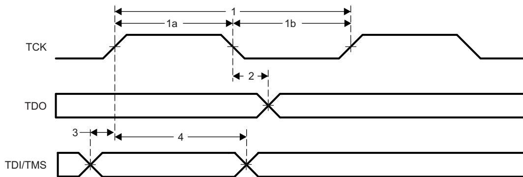
Figure 5-101. JTAG Timing
