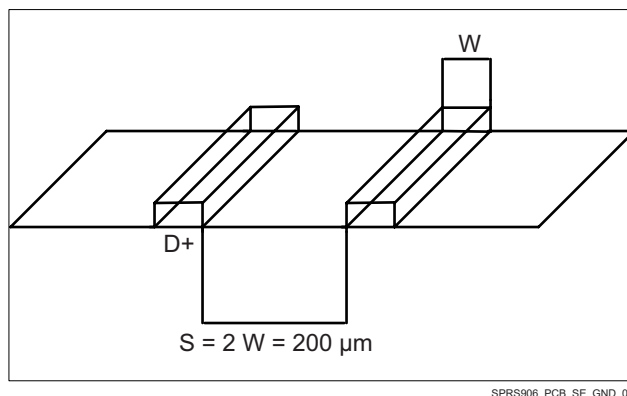
Figure 7-19. Ground Guard Illustration
