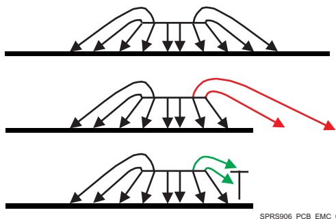
Figure 7-12. Field Lines of a Signal Above Ground
