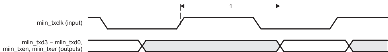
Figure 5-64. GMAC Transmit Interface Timing MIIn operation
