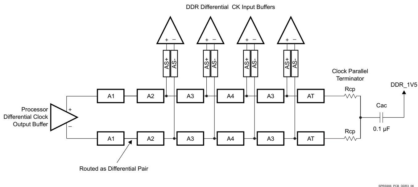
Figure 7-42. CK Topology for Four x8 DDR3 Devices
