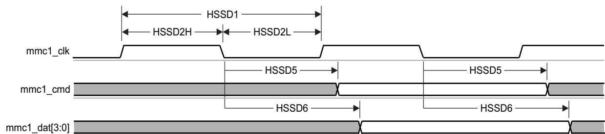
Figure 7-57. MMC/SD/SDIO in - High Speed - Transmitter Mode
