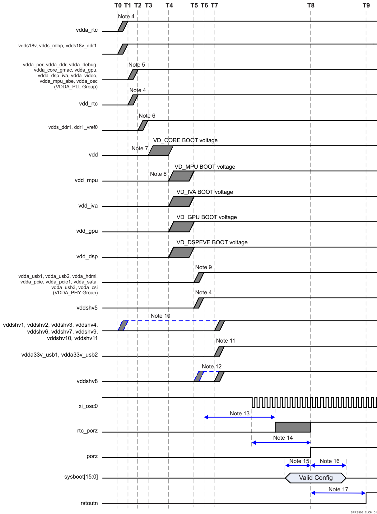
Figure 5-2. Recommended Power-Up Sequencing
