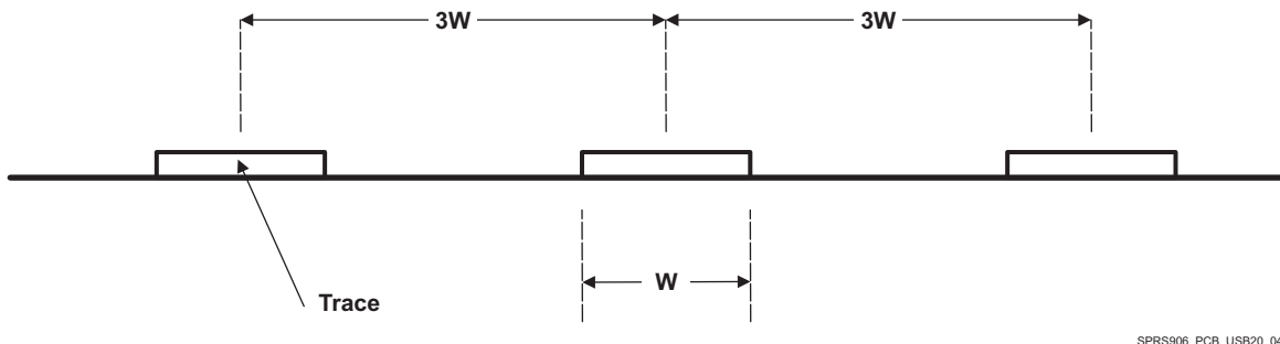
Figure 8-24. 3W Spacing Rule
