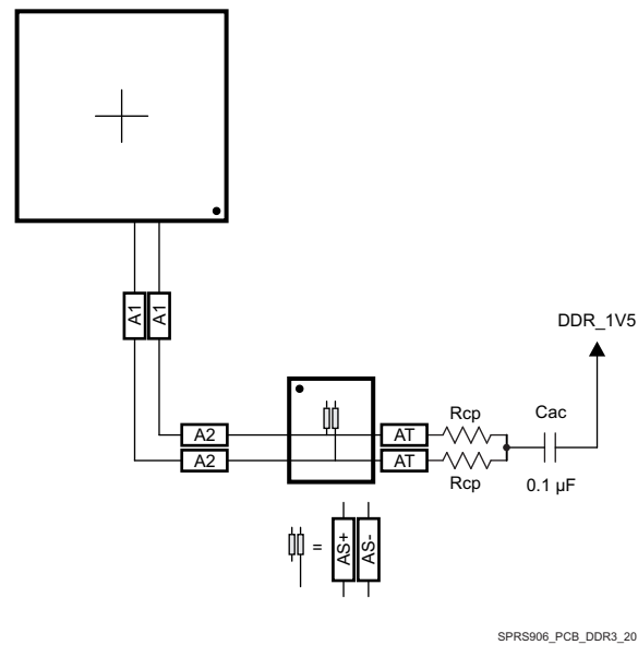
Figure 8-59. CK Routing for One DDR3 Device
