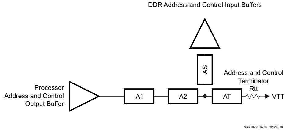
Figure 8-58. ADDR_CTRL Topology for One DDR3 Device
