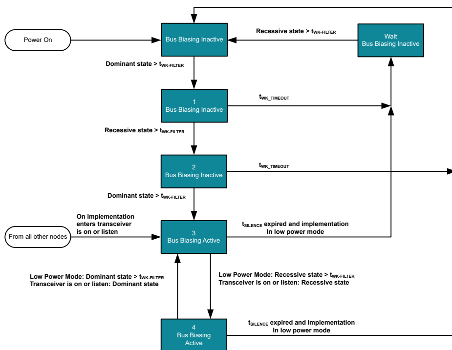
Figure 8-10. Automatic bus biasing state diagram
