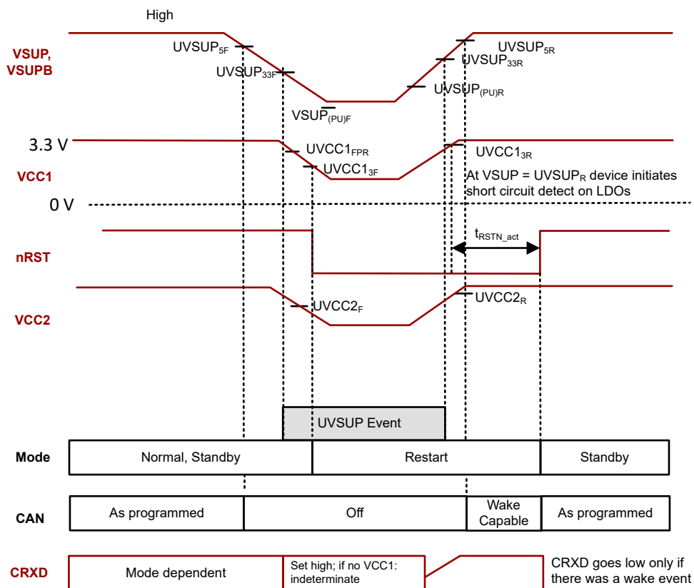
Figure 10-5. Brownout Above VSUP (PIU)F for VCC1= 3.3V
