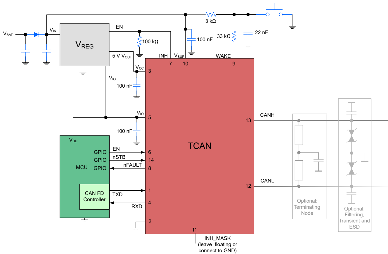
Simplified Schematic
