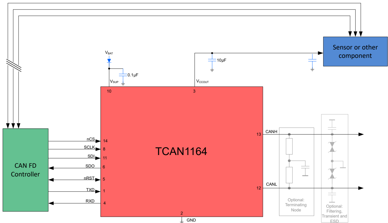
Figure 11-1. Typical Application
