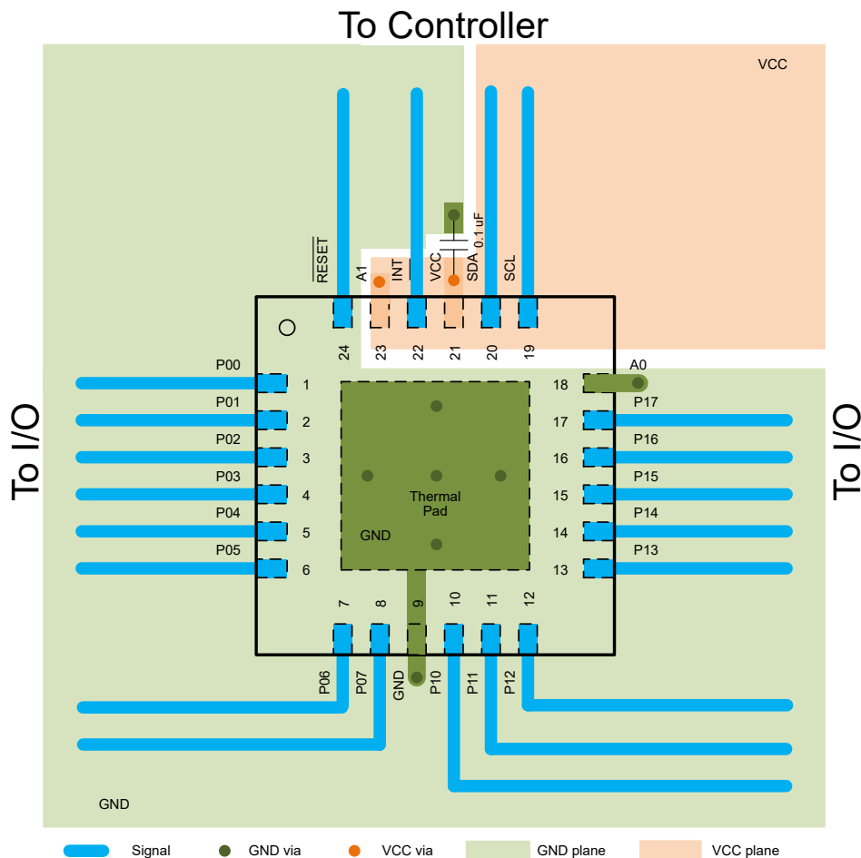
Figure 8-9. TCAL6416 Layout
