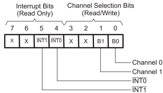
Figure 15. Control Register
