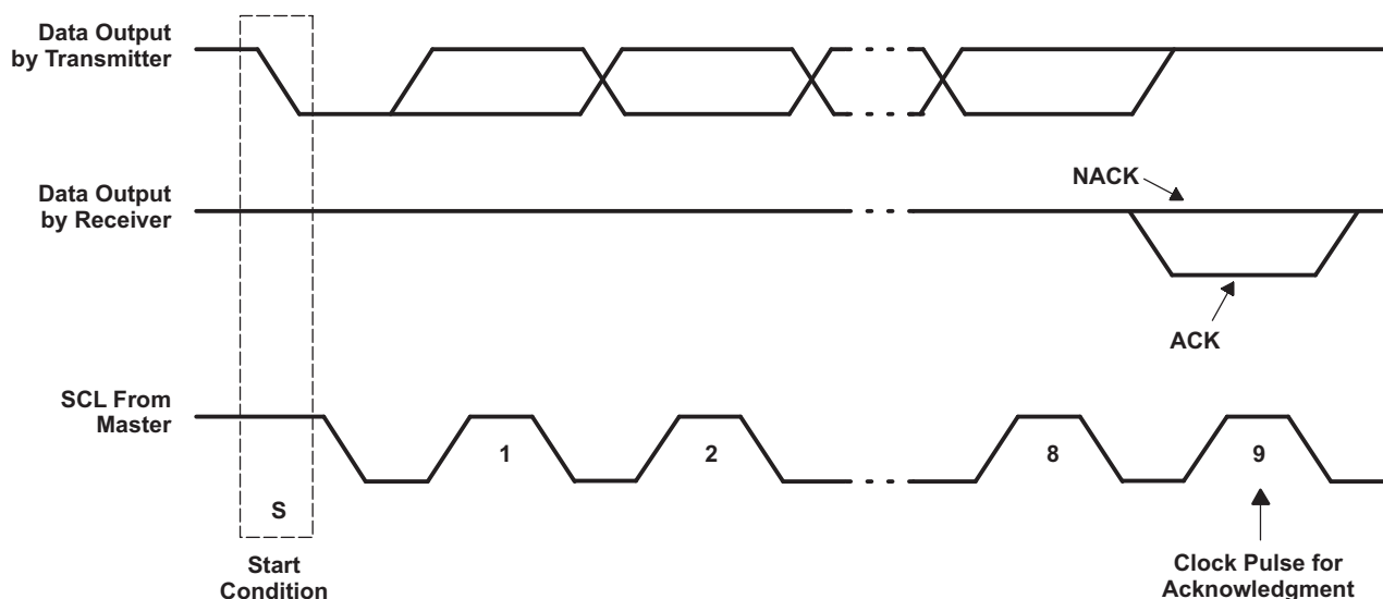
Figure 11. Acknowledgment on I²C Bus
