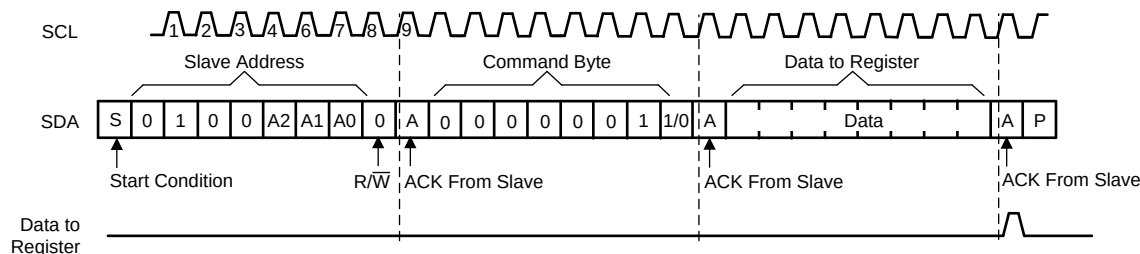
Figure 30. Write to Configuration or Polarity Inversion Registers
