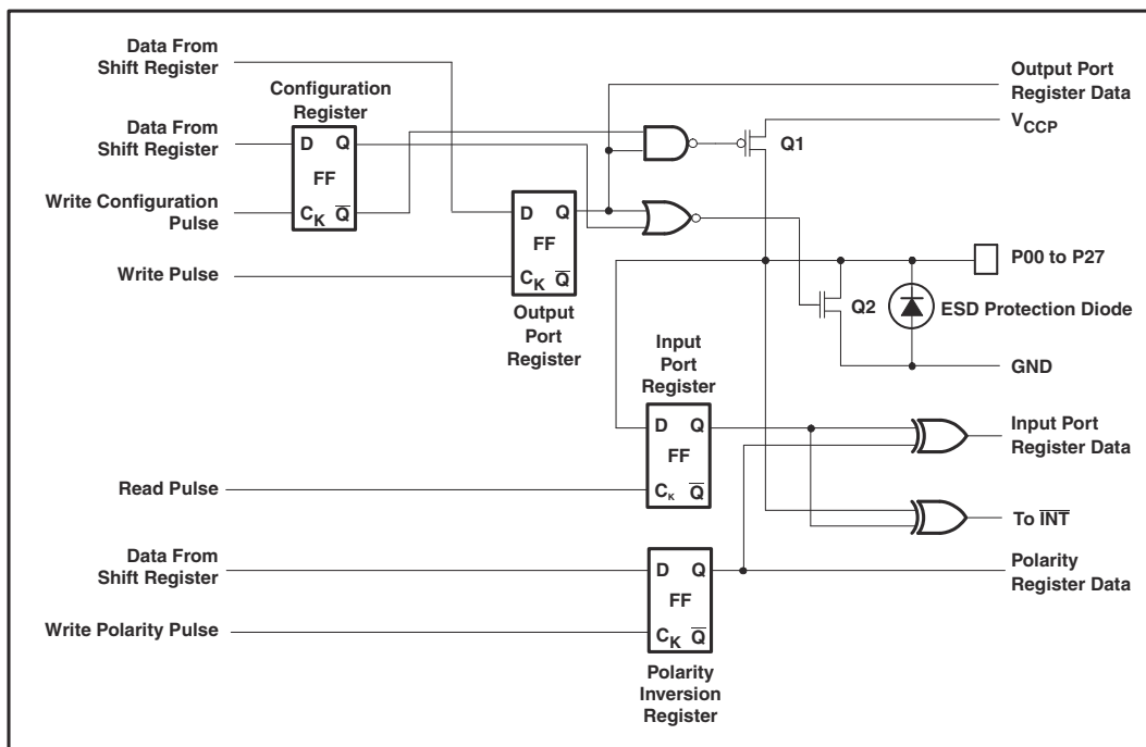
Figure 8-1. Positive Logic
