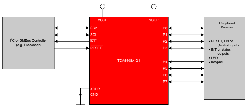
Simplified Schematic
