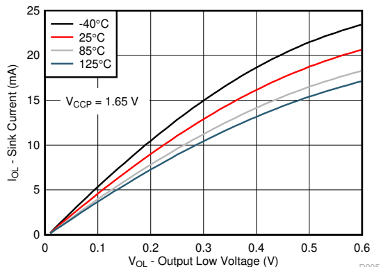
Figure 6-5. I/O Sink Current vs Output Low Voltage ( V_{CCP} = 1.65\text{ V} )
