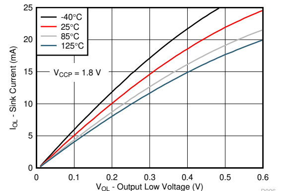
Figure 6-6. I/O Sink Current vs Output Low Voltage ( V_{CCP} = 1.8\text{ V} )
