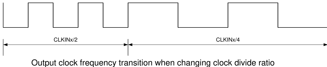
Figure 15. CLK Divide Ratio Change on Card CLK Output
