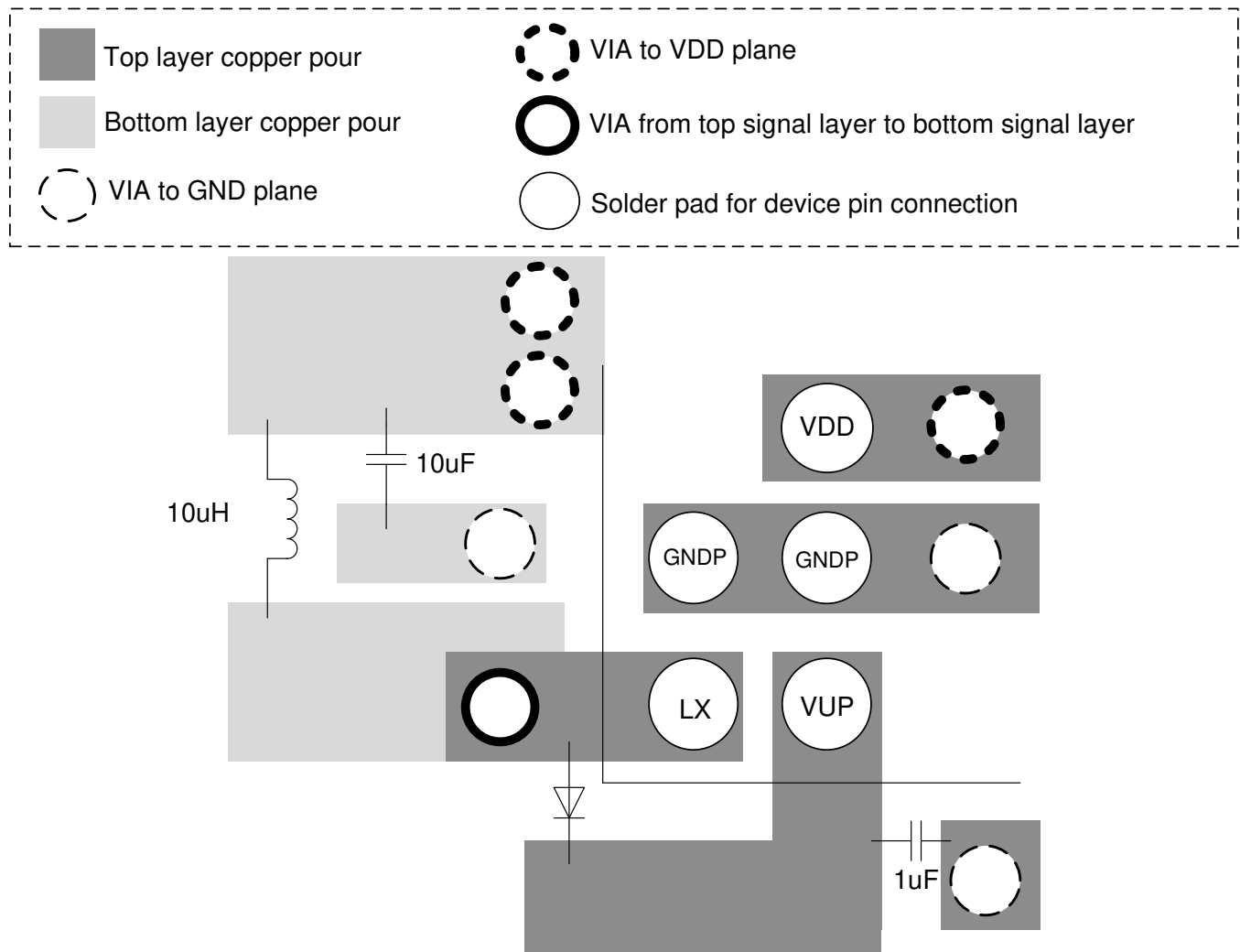
Figure 28. Example Layout of DC-DC Boost Section of TCA5013
