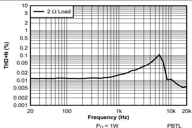
Figure 7-38. THD+N vs Frequency - PBTL - 384 kHz
