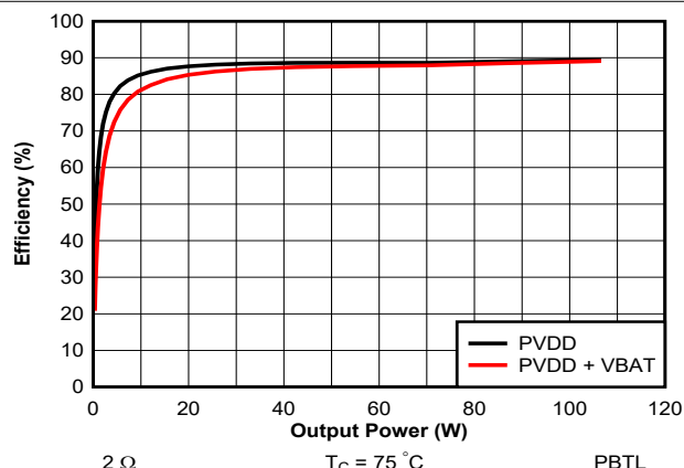
Figure 7-40. Efficiency vs Output Power - PBTL - 2 \Omega - 384 kHz
