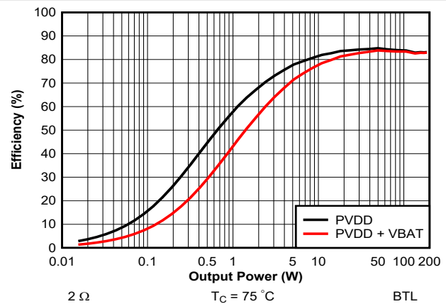
Figure 7-26. Efficiency vs Output Power - 2 \Omega - 384 kHz (Zoomed)
