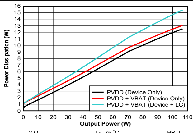
Figure 7-42. Power Dissipation vs Output Power - PBTL - 2 \Omega - 384 kHz
