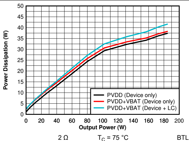
Figure 7-11. Power Dissipation vs Output Power - 14.4 V - 2 \Omega
