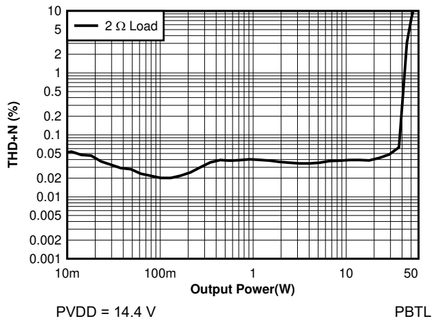
Figure 7-28. THD+N vs Power - PBTL - 14.4V
