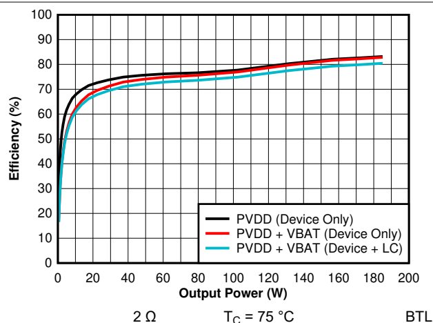
Figure 7-9. Efficiency vs Output Power - 14.4 V - 2 \Omega
