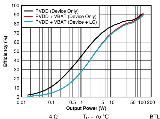
Figure 7-7. Efficiency vs Output Power - 14.4 V - 4 \Omega (Zoomed)
