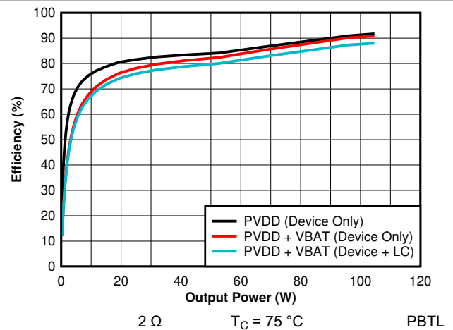
Figure 7-33. Efficiency vs Output Power - PBTL - 2 \Omega
