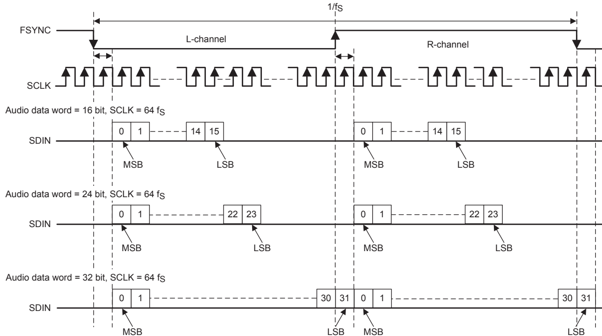
Figure 9-4. I²S Audio Data Format
