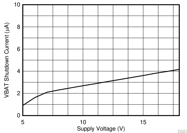
Figure 7-21. VBAT Standby Current vs Voltage
