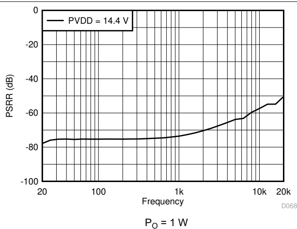
Figure 7-3. VBAT + PVDD PSRR vs Frequency
