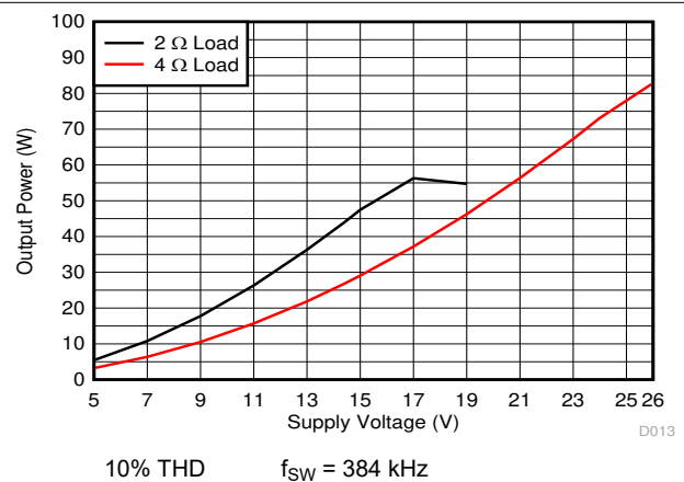
Figure 7-12. Output Power vs Supply Voltage
