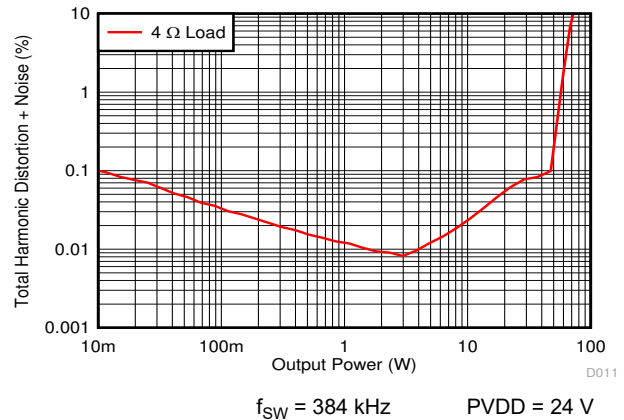
Figure 7-10. THD+N vs Power
