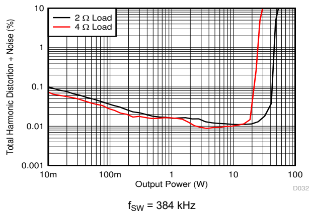
Figure 7-26. PBTL THD+N vs Power
