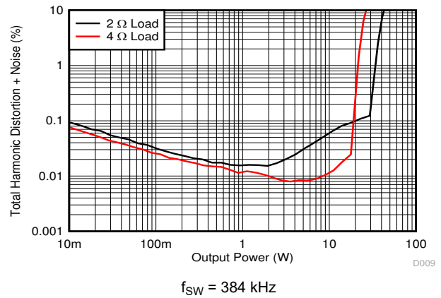
Figure 7-8. THD+N vs Power
