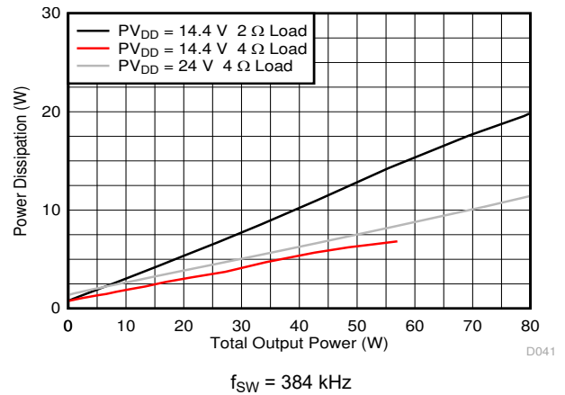
Figure 7-32. BTL Power Dissipation vs Total Output Power
