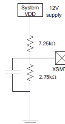
Figure 45. External Power Sense
