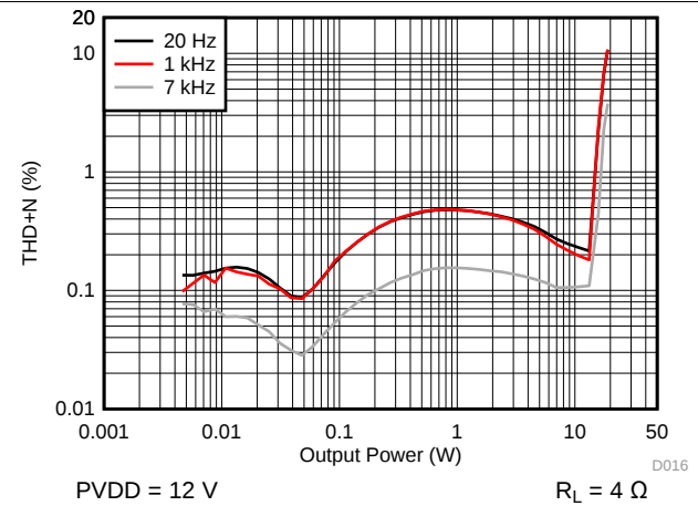
Figure 20. THD+N vs Output Power - PBTL
