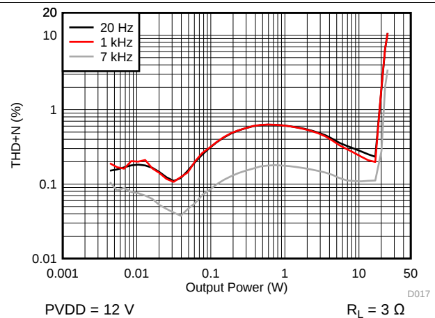
Figure 21. THD+N vs Output Power - PBTL
