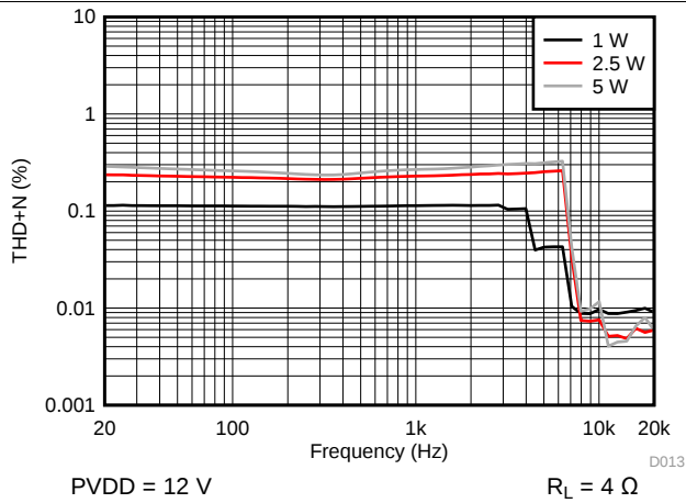
Figure 17. THD+N vs Frequency - PBTL
