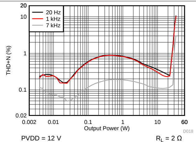
Figure 22. THD+N vs Output Power - PBTL
