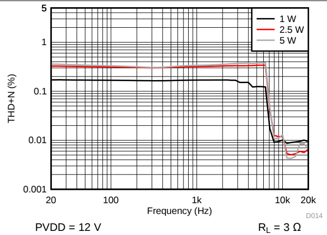
Figure 18. THD+N vs Frequency - PBTL
