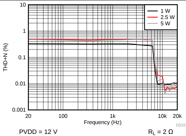
Figure 19. THD+N vs Frequency - PBTL
