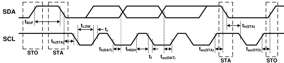
Figure 6-1. I²C Timing Diagram
