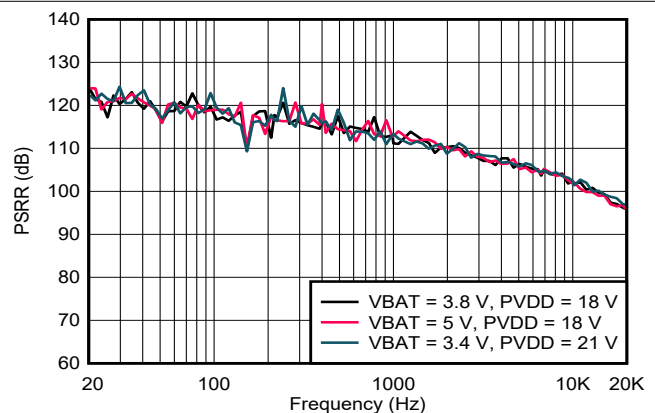
Figure 6-18. AVDD PSRR vs Frequency
