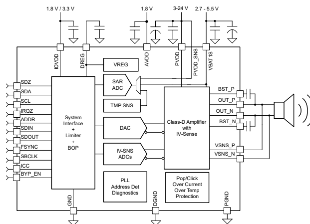
Schematic
