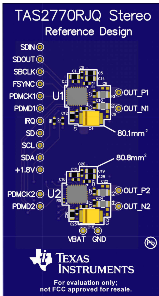
Figure 11-2. Stereo EVM Layout Reference Design - 01
