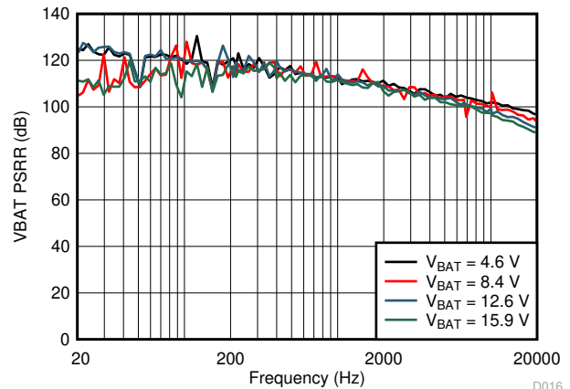
Figure 6-16. VBAT PSRR vs Frequency
