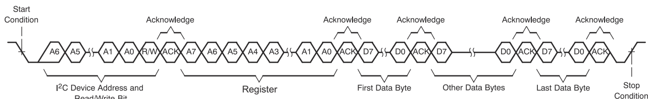
Figure 8-3. Multi-Byte Write Transfer
