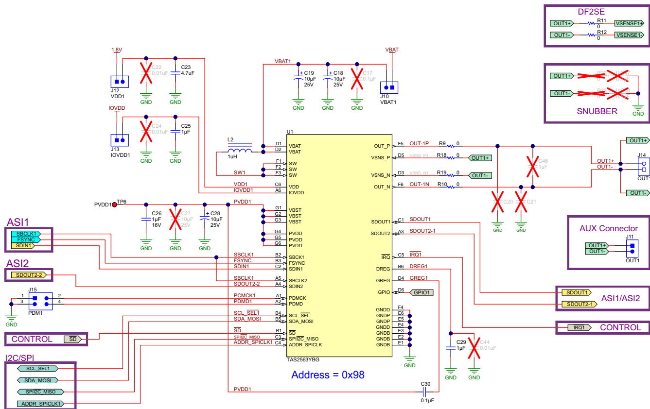
Figure 6-1. TAS2563 Circuit
