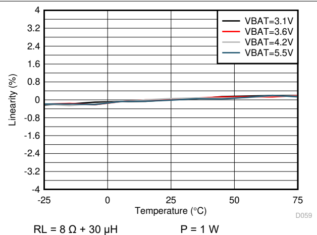
Figure 5-56. V-sense Linearity vs Temperature
