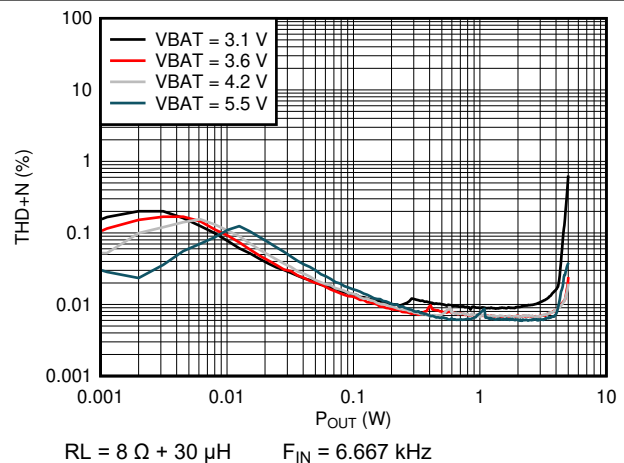
Figure 5-14. THD+N vs Output Power (QFN Package)
