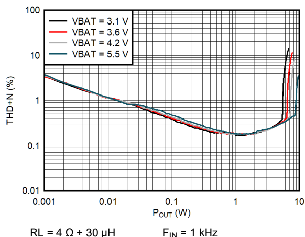
Figure 5-38. I-sense THD+N vs Output Power (QFN Package)
