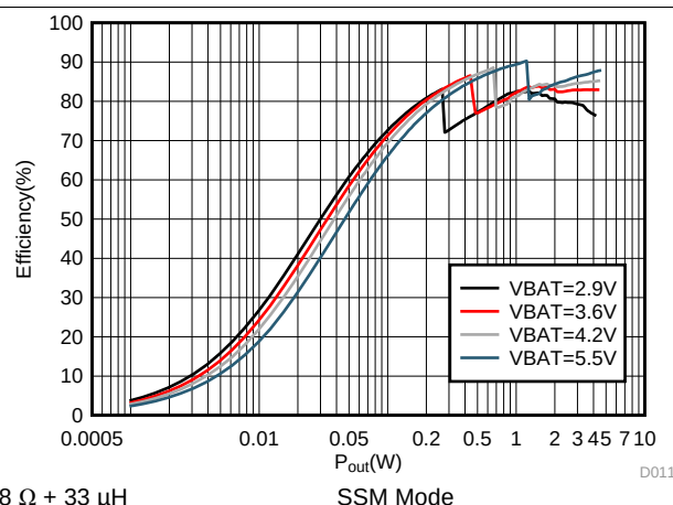
Figure 17. Efficiency vs Output Power High Efficiency
