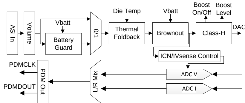
Figure 54. Mode 3 Processing Block Diagram
