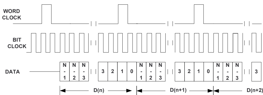
Figure 46. Timing Diagram for Mono PCM Mode with ASI_OFFSET1=2
