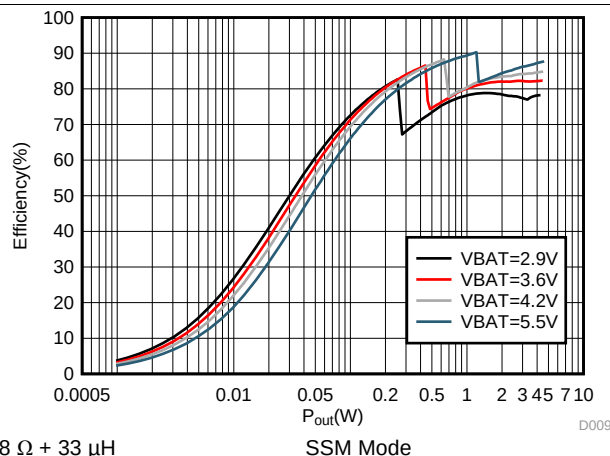
Figure 15. Efficiency vs Output Power Low Inrush
