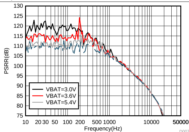
Figure 13. VBAT Supply Ripple Rejection vs Frequency
