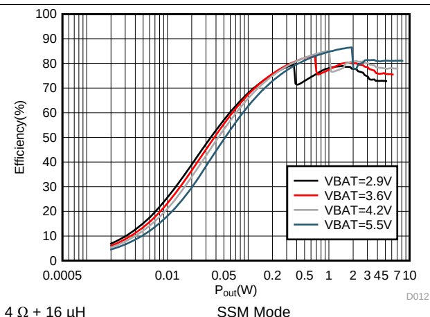
Figure 18. Efficiency vs Output Power High Efficiency
