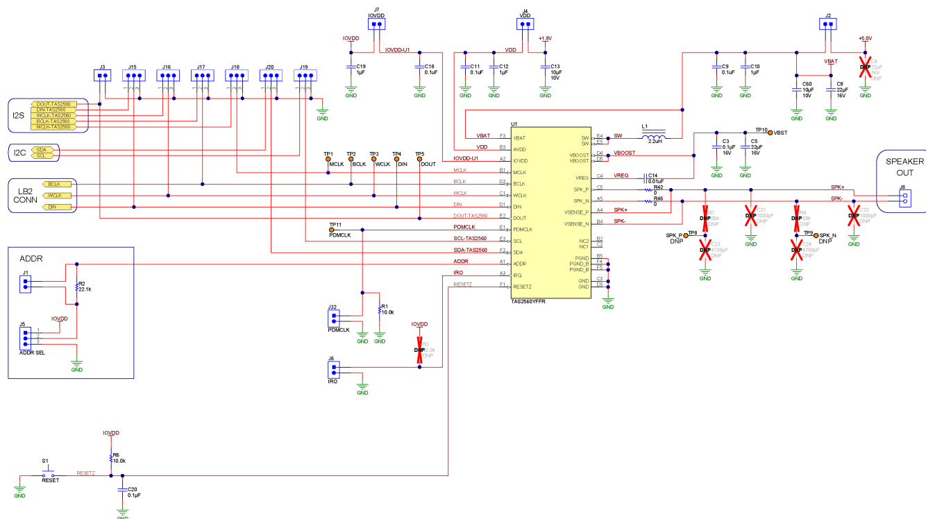
Figure 23. TAS2560 Test Circuit
