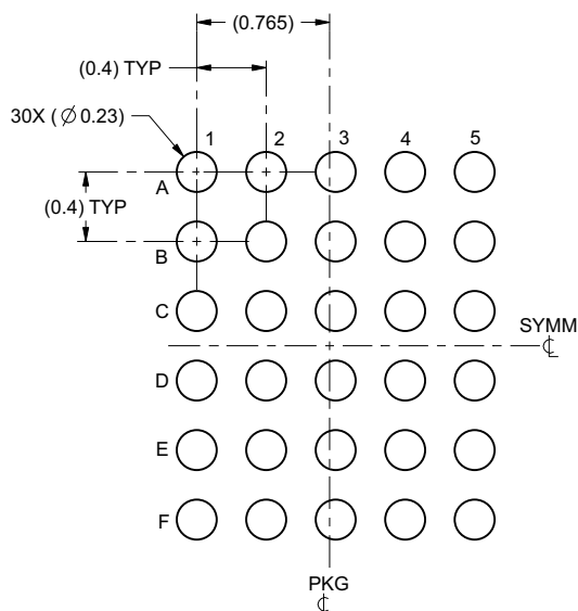
LAND PATTERN EXAMPLE SCALE:25X
