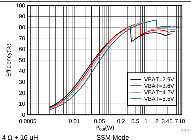
Figure 16. Efficiency vs Output Power Low Inrush
