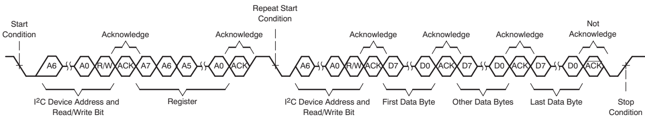
Figure 29. Multiple-Byte Read Transfer
