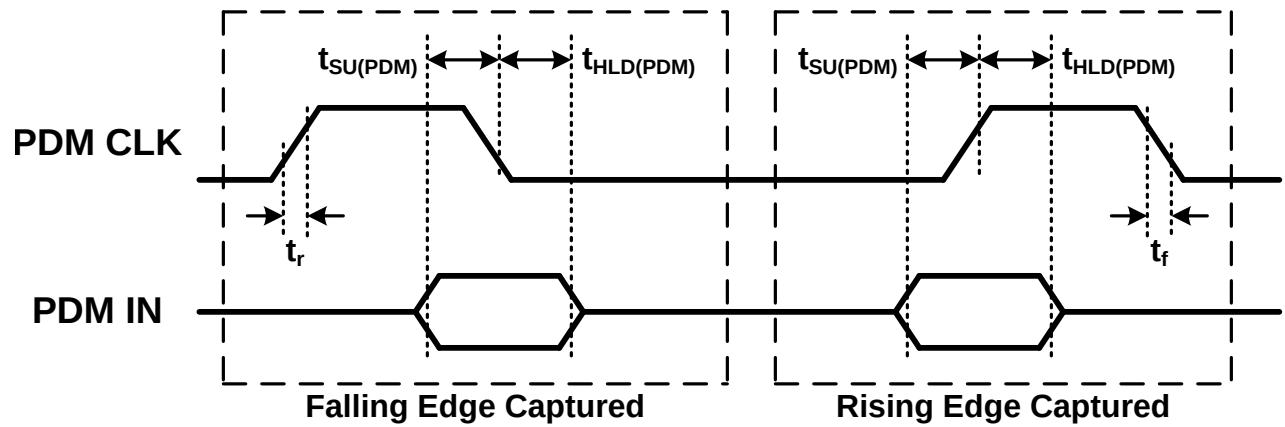
Figure 6. PDM Timing
