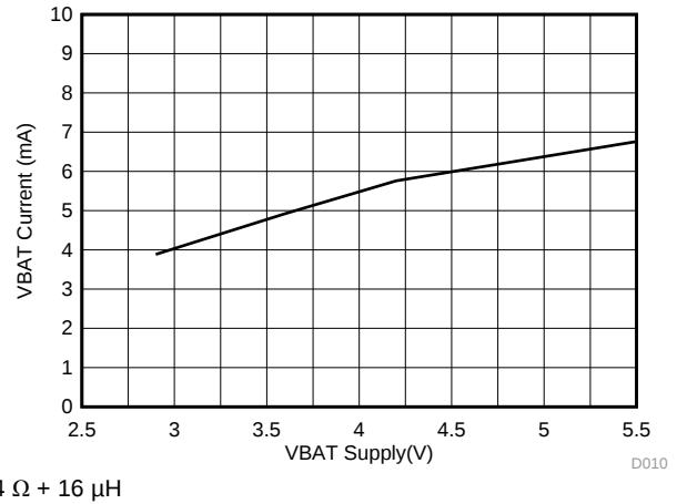
Figure 16. Quiescent Current vs VBAT
