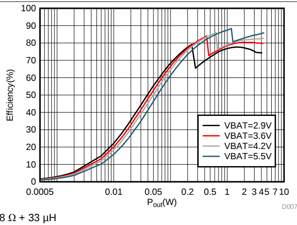
Figure 13. Efficiency vs Output Power
