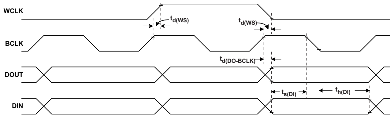
Figure 5. DSP Timing in Master Mode
