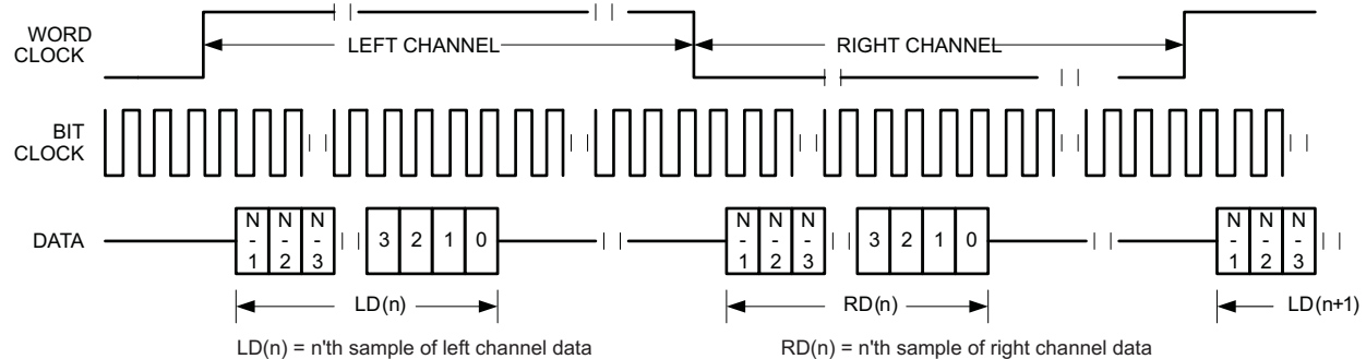
Figure 37. Timing Diagram for Left-Justified Mode with ASI_OFFSET1 = 1
