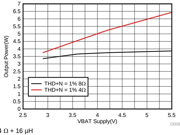
Figure 15. Output Power for 1% THD+N vs VBAT
