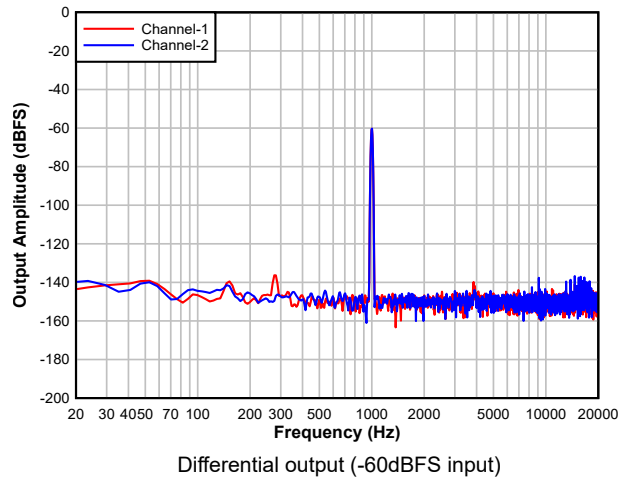
Figure 8-2. DAC FFT with -60dBFS Input
