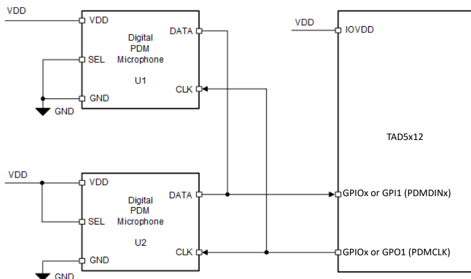
Figure 6-18. Digital PDM Microphones Connection Diagram for the TAD5212
