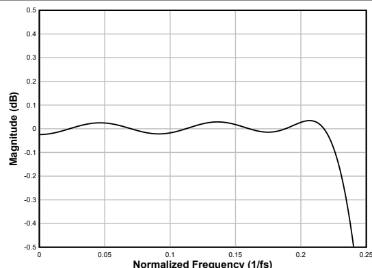
Figure 6-75. Linear-phase Decimation Filter Pass-Band Ripple
