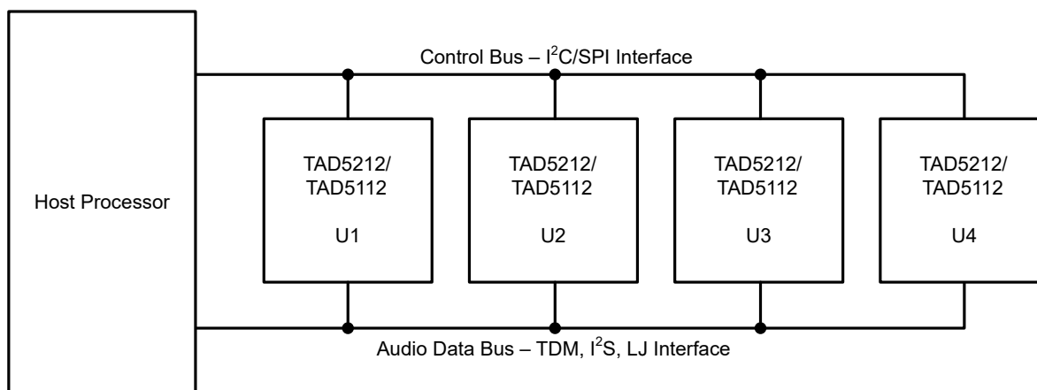
Figure 6-13. Multiple TAD5212 Devices With Shared Control and Audio Data Buses
