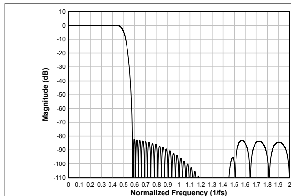
Figure 6-32. Linear-phase Interpolation Filter Magnitude Response
