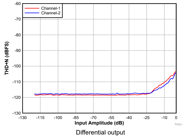
Figure 8-3. DAC THD+N Level vs Input
