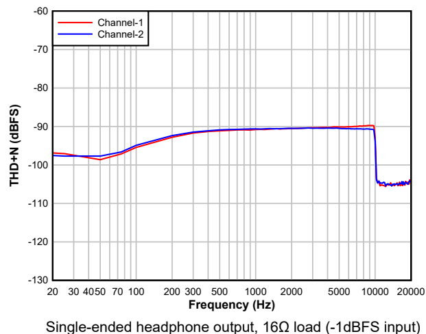
Figure 5-14. DAC THD+N Level vs Frequency
