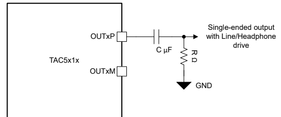
Figure 6-15. Mono Single-ended Output Connection on OUT1P (OUT1x_CFG[2:0] = 3'b010)
