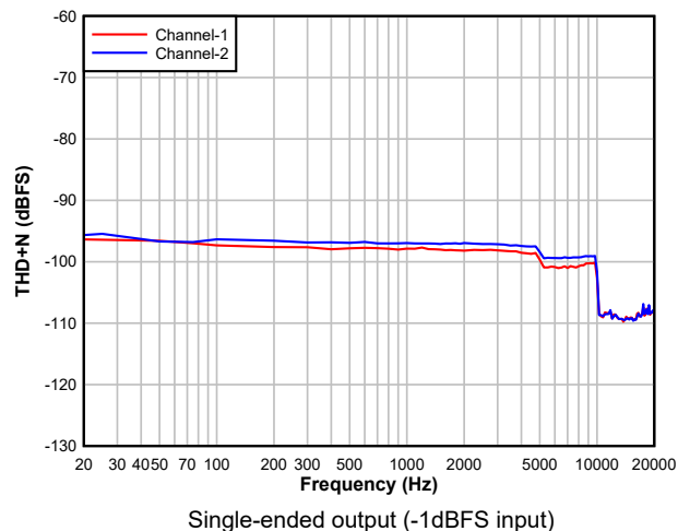
Figure 5-12. DAC THD+N Level vs Frequency
