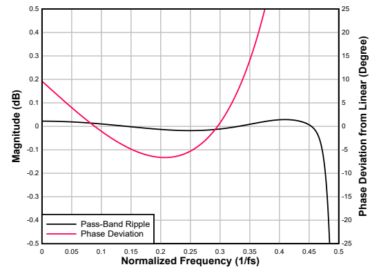
Figure 6-97. Ultra Low-latency Decimation Filter Pass-Band Ripple and Phase Deviation
