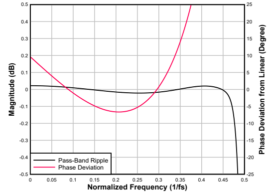
Figure 6-95. Ultra Low-latency Decimation Filter Pass-Band Ripple and Phase Deviation
