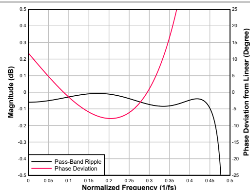
Figure 6-53. Ultra-Low-Latency interpolation Filter Pass-Band Ripple and Phase Deviation
