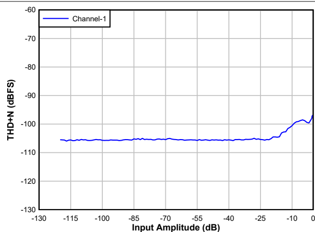
Figure 5-20. DAC THD+N Level vs Input
