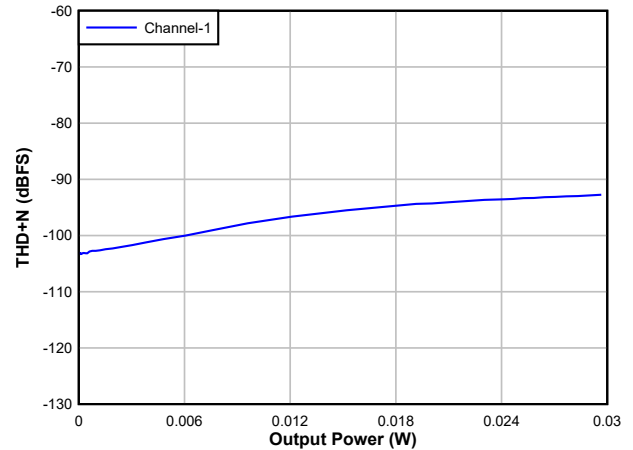
Pseudo-differential headphone output, 16Ω load
