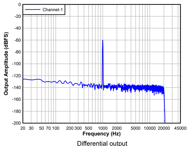
Figure 5-30. DAC FFT with -60dBFS Input
