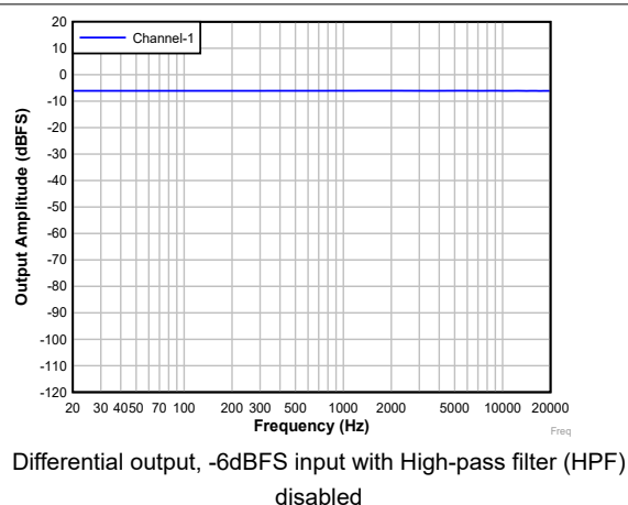
Figure 5-34. DAC Frequency Response
