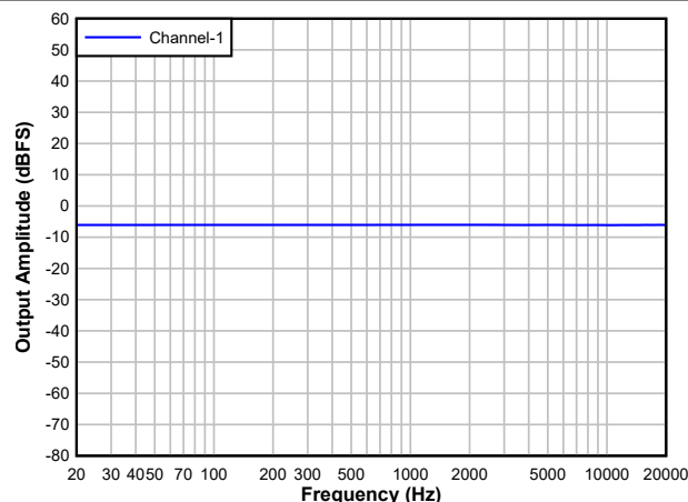
Figure 5-11. ADC Frequency Response
