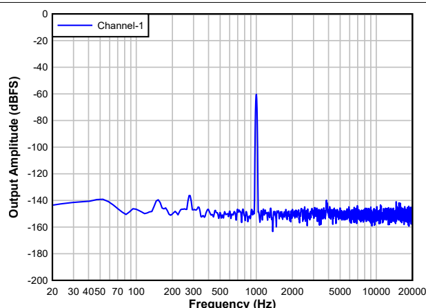
Figure 8-4. ADC FFT with -60dBFS Input
