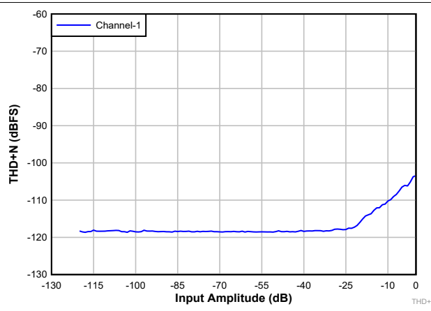
Figure 8-7. DAC THD+N Level vs Input
