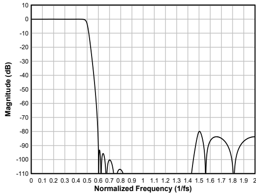
Figure 6-84. Low-latency Interpolation Filter Magnitude Response
