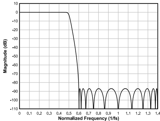
Figure 6-86. Low-latency Interpolation Filter Magnitude Response
