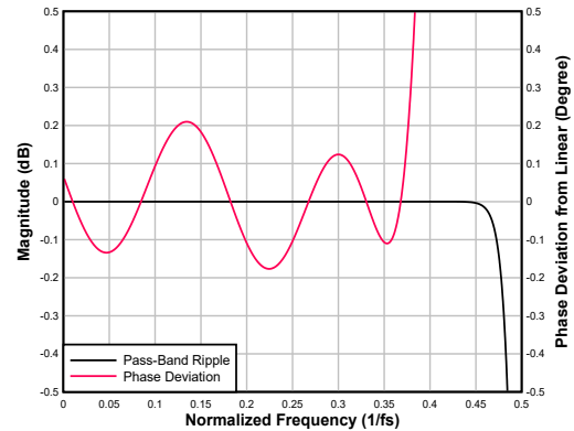
Figure 6-87. Low-latency Interpolation Filter Pass-Band Ripple and Phase Deviation
