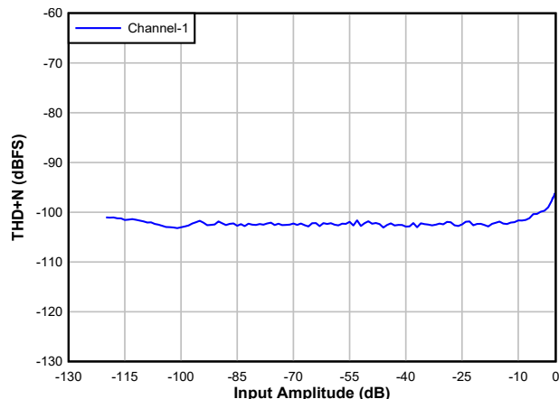
Figure 8-3. ADC THD+N Level vs Input
