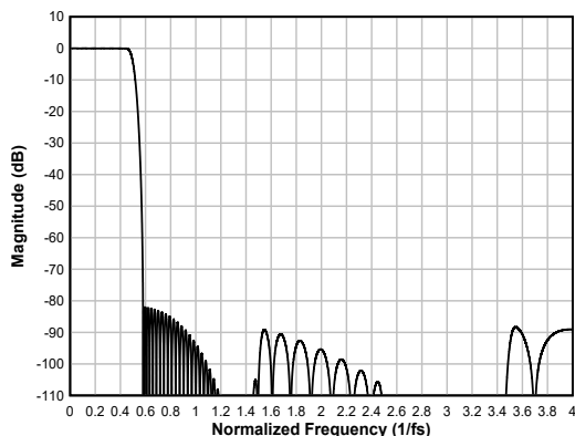
Figure 6-72. Linear-phase Interpolation Filter Magnitude Response
