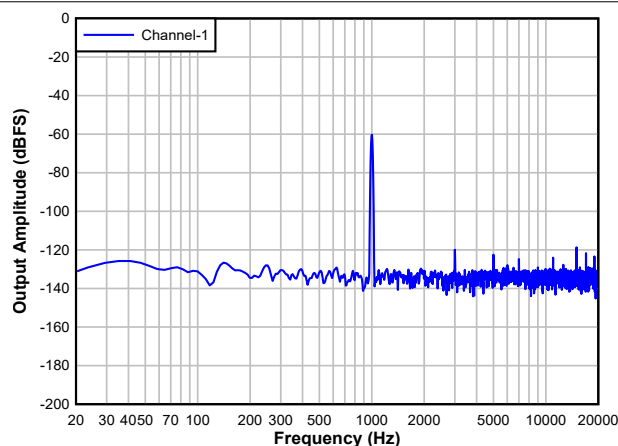
Figure 8-2. ADC FFT with -60dBFS Input
