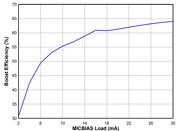
Figure 5-18. Boost Efficiency vs MICBIAS Load Current
