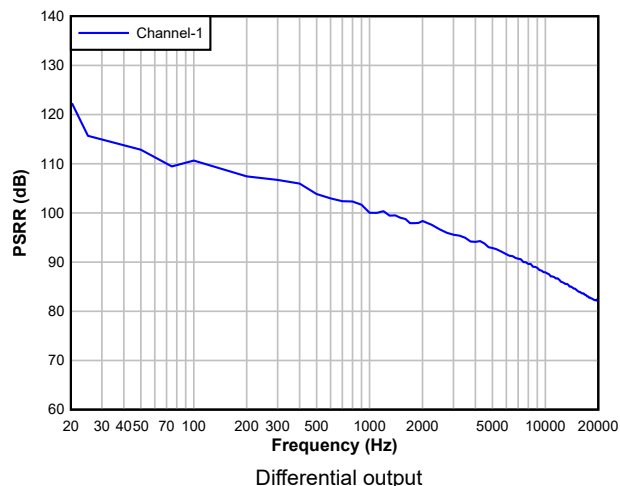
Figure 5-32. DAC PSRR vs Frequency
