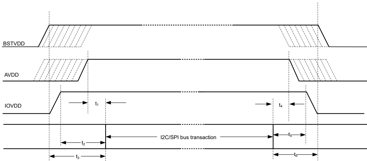
Figure 8-8. Power-Supply Sequencing Requirement Timing Diagram
