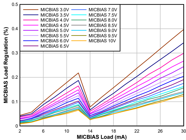
Figure 5-17. MICBIAS Load Regulation
