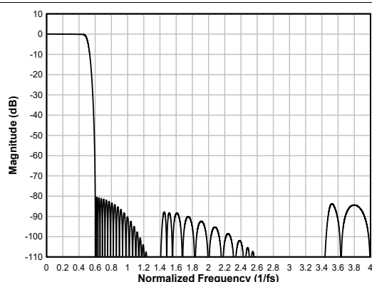
Figure 6-66. Linear-phase Interpolation Filter Magnitude Response
