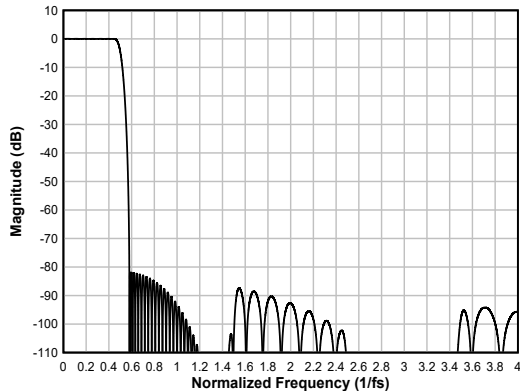
Figure 6-70. Linear-phase Interpolation Filter Magnitude Response
