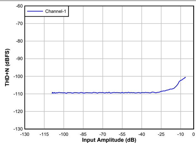
Figure 5-19. DAC THD+N Level vs Input
