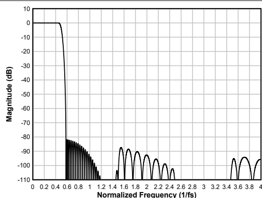
Figure 6-68. Linear-phase Interpolation Filter Magnitude Response
