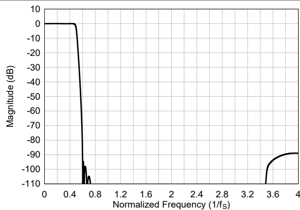
Figure 6-89. Ultra-Low-Latency interpolation Filter Magnitude Response
