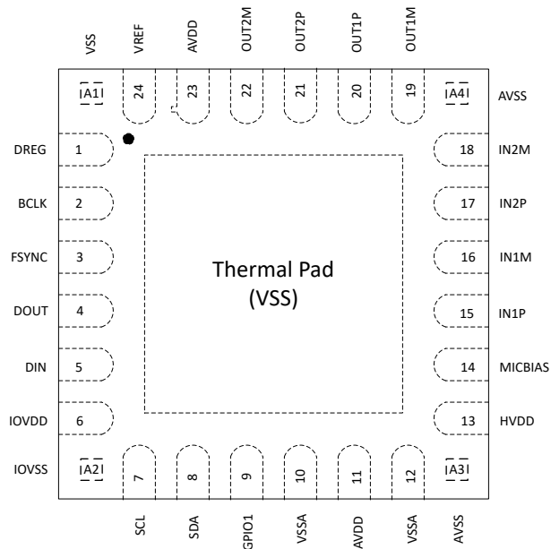
Figure 4-1. TAC5301-Q1 24-Pin QFN Package with Exposed Thermal Pad and Corner Pins, Top View
