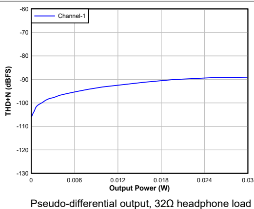
Figure 5-19. DAC THD+N Level vs output power
