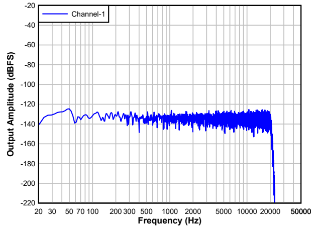
Figure 5-10. ADC FFT with Idle Channel Input
