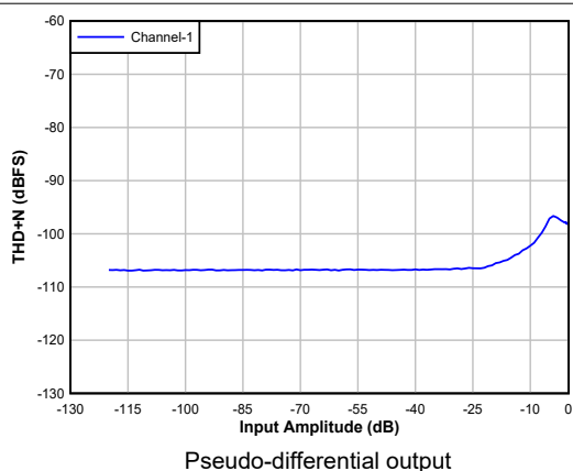
Figure 5-17. DAC THD+N Level vs Input
