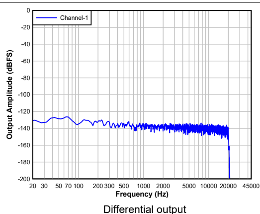
Figure 5-23. DAC FFT with Idle Channel Input
