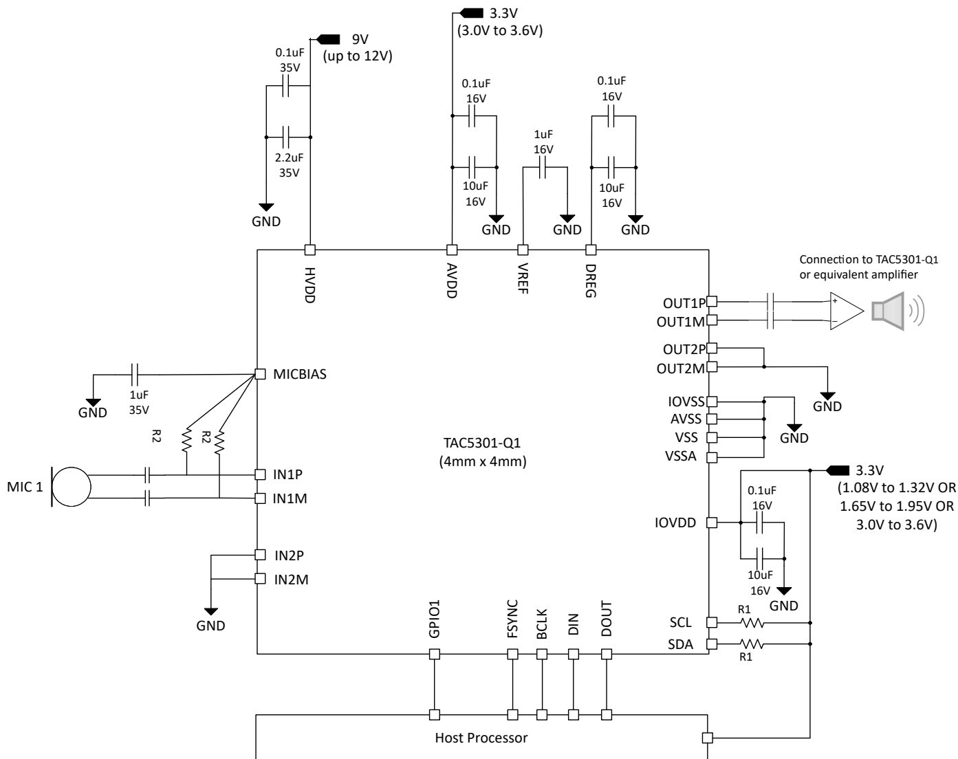
Figure 8-1. Mono Microphone with Mono Lineout Block Diagram
