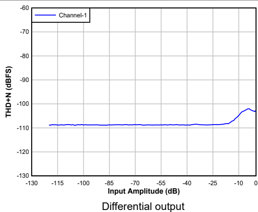
Figure 5-15. DAC THD+N Level vs Input
