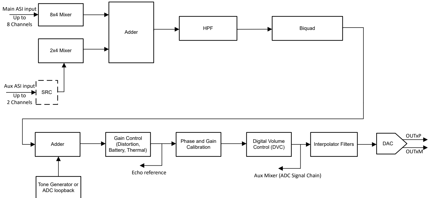
Figure 6-61. DAC Signal-Chain Processing Flowchart
