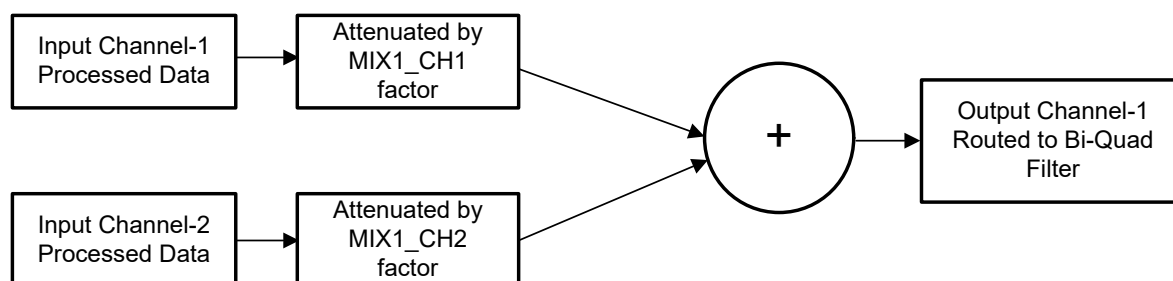
Figure 6-25. Programmable Digital Mixer Block Diagram
