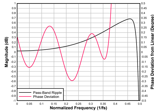
Figure 6-41. Low-latency Decimation Filter Pass-Band Ripple and Phase Deviation
