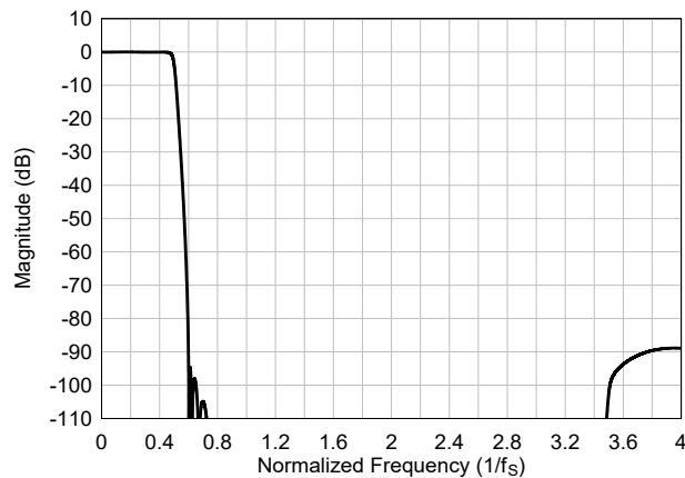
Figure 6-91. Ultra-Low-Latency interpolation Filter Magnitude Response
