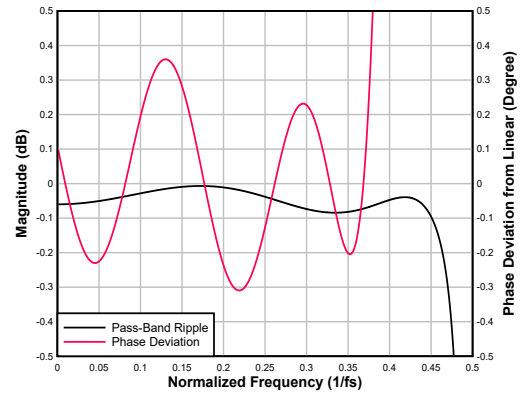
Figure 6-80. Low-latency Interpolation Filter Pass-Band Ripple and Phase Deviation
