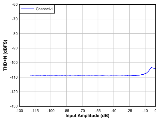
Figure 8-2. ADC THD+N Level vs Input
