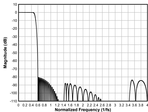
Figure 6-63. Linear-phase Interpolation Filter Magnitude Response
