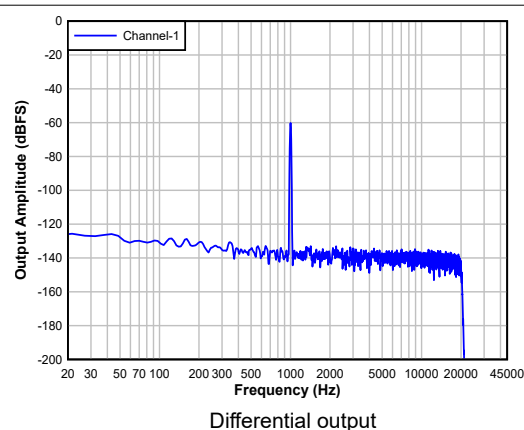
Figure 5-24. DAC FFT with -60dBFS Input
