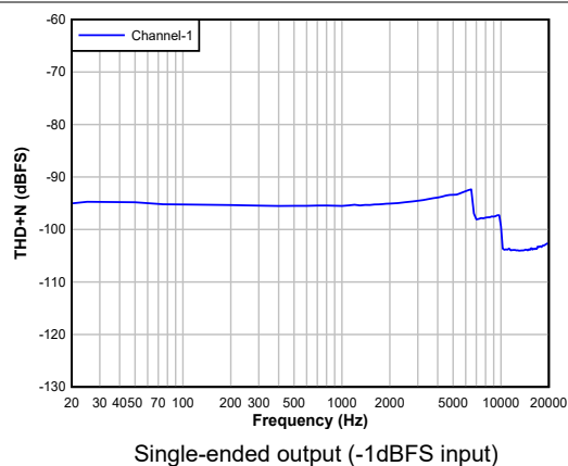
Figure 5-21. DAC THD+N Level vs Frequency
