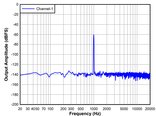
Figure 8-5. DAC FFT with -60dBFS Input
