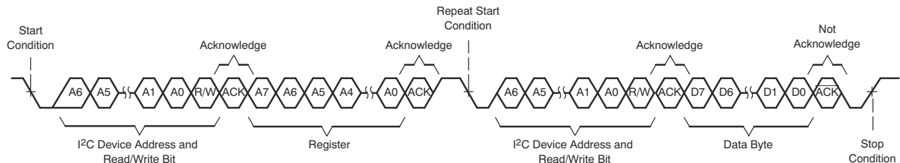
Figure 6-100. I 2 C Single-Byte Read Transfer
