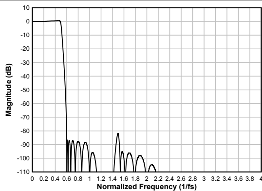
Figure 6-50. Ultra Low-latency Decimation Filter Magnitude Response
