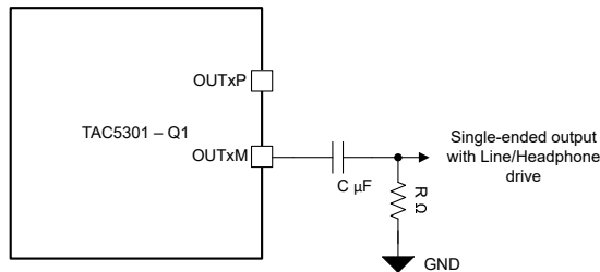
Figure 6-21. Mono Single-ended Output Connection on OUT1M (OUT1x_CFG[2:0] = 3'b011)
