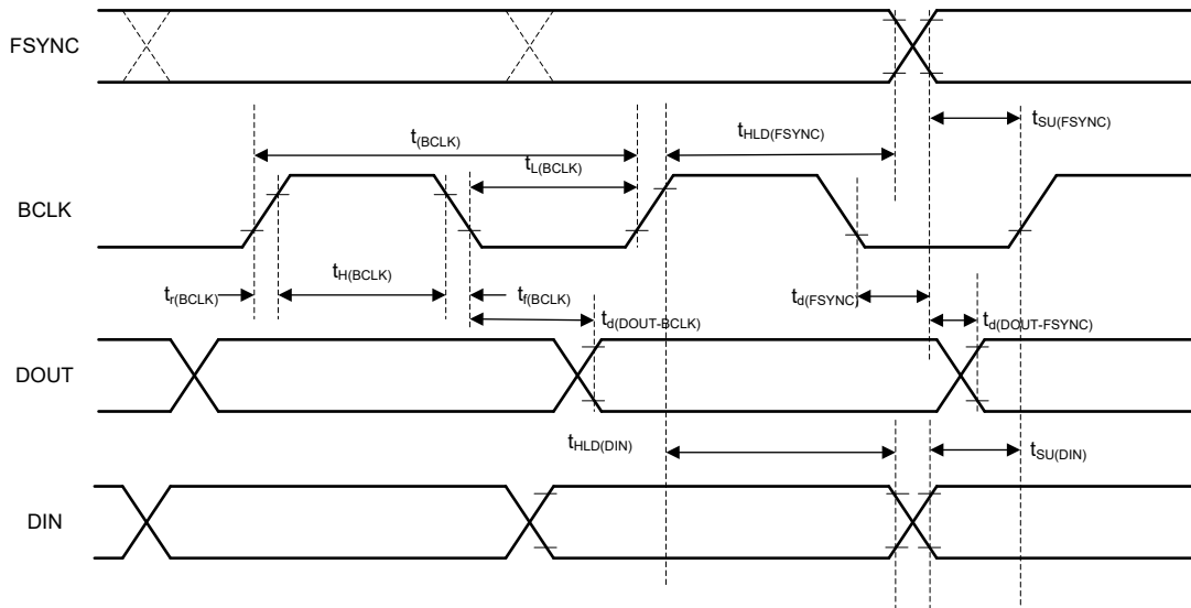
Figure 5-2. TDM (With BCLK_POL = 1), I 2 S, and LJ Interface Timing Diagram
