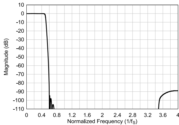
Figure 6-87. Ultra-Low-Latency interpolation Filter Magnitude Response
