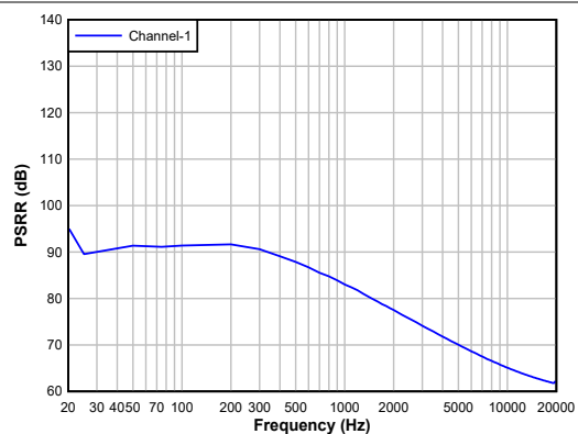
Figure 5-27. DAC PSRR vs Frequency
