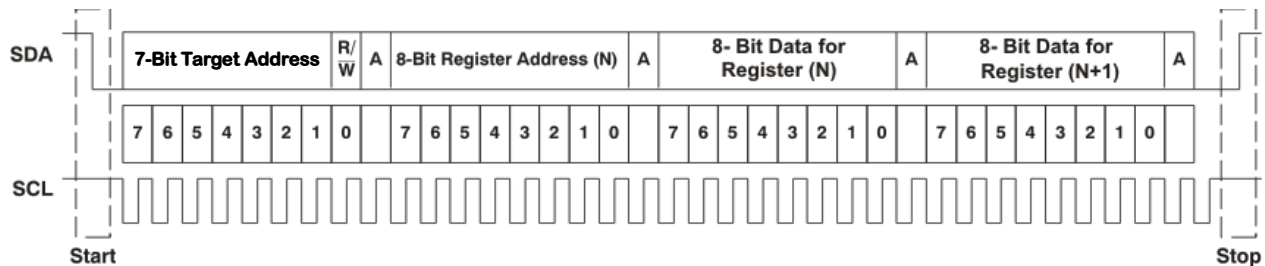
Figure 6-97. Typical I 2 C Sequence
