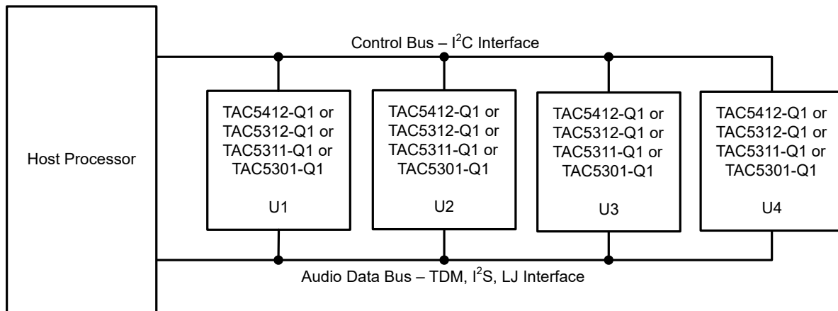
Figure 6-14. Multiple TAC5301-Q1 Devices With Shared Control and Audio Data Buses
