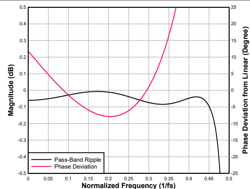
Figure 6-90. Ultra-Low-Latency interpolation Filter Pass-Band Ripple and Phase Deviation
