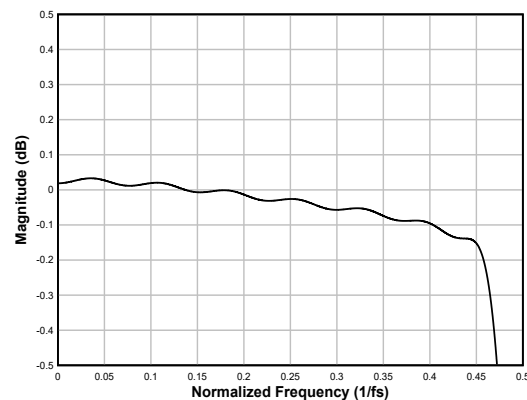
Figure 6-64. Linear-phase Interpolation Filter Pass-Band Ripple
