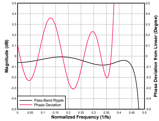
Figure 6-78. Low-latency Interpolation Filter Pass-Band Ripple and Phase Deviation
