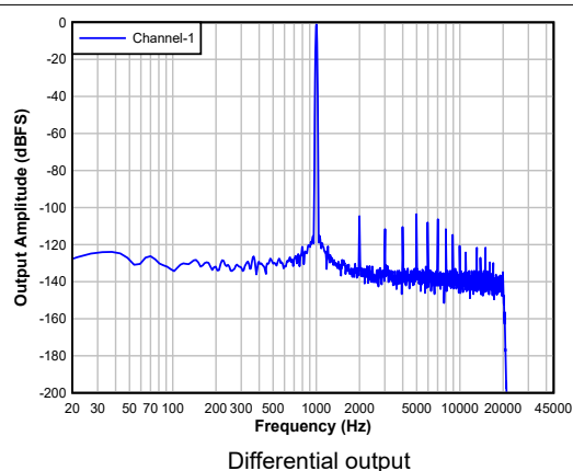
Figure 5-25. DAC FFT with -1dBFS Input
