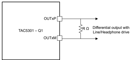
Figure 6-19. Differential Output Connection (OUT1x_CFG[2:0] = 3'b000)
