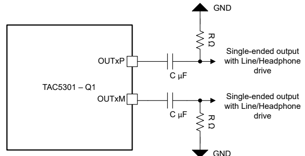
Figure 6-22. Stereo Single-ended Output Connection (OUT1x_CFG[2:0] = 3'b001)
