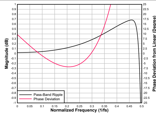
Figure 6-51. Ultra Low-latency Decimation Filter Pass-Band Ripple and Phase Deviation
