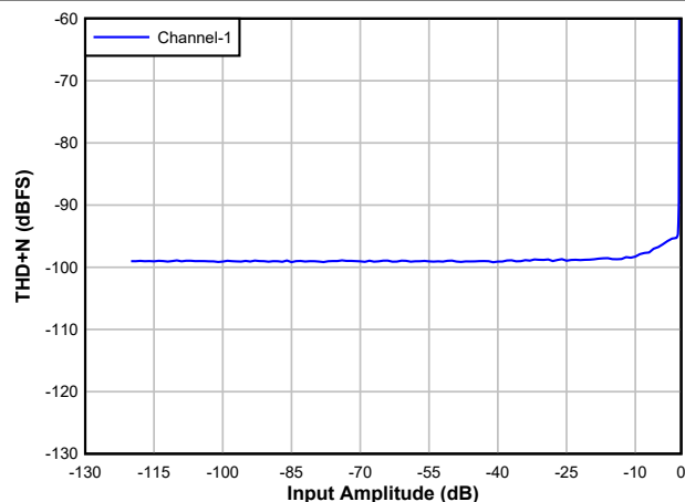
Figure 5-3. ADC THD+N Level vs Input
