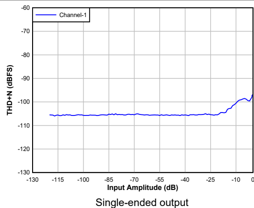
Figure 5-16. DAC THD+N Level vs Input
