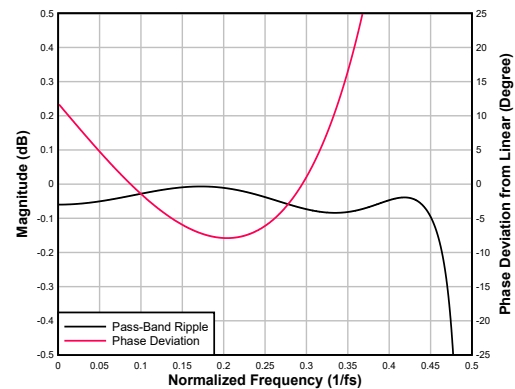
Figure 6-92. Ultra-Low-Latency interpolation Filter Pass-Band Ripple and Phase Deviation
