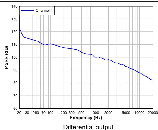
Figure 5-26. DAC PSRR vs Frequency
