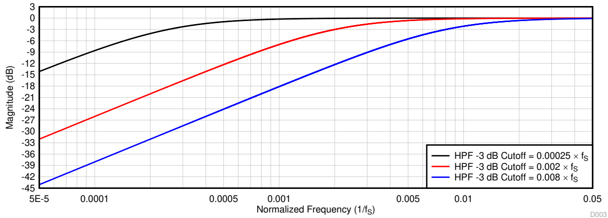
Figure 6-24. HPF Filter Frequency Response Plot
