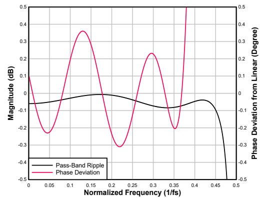
Figure 6-82. Low-latency Interpolation Filter Pass-Band Ripple and Phase Deviation
