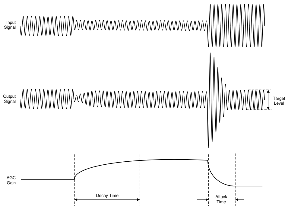
Figure 6-60. AGC Characteristics
