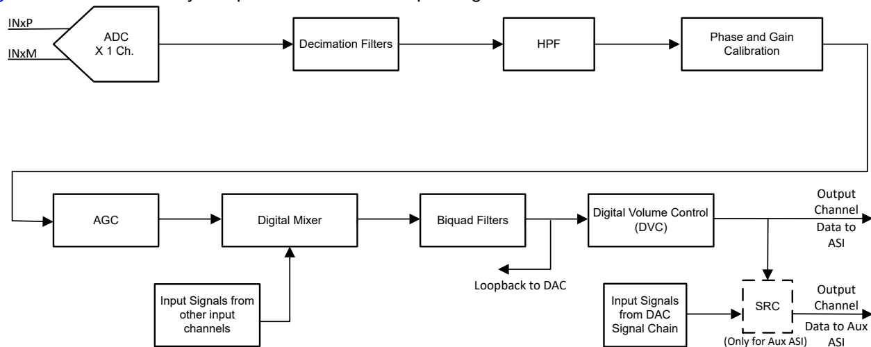
Figure 6-23. ADC Signal-Chain Processing Flowchart
