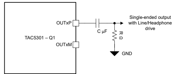
Figure 6-20. Mono Single-ended Output Connection on OUT1P (OUT1x_CFG[2:0] = 3'b010)
