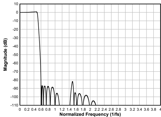
Figure 6-40. Low-latency Decimation Filter Magnitude Response
