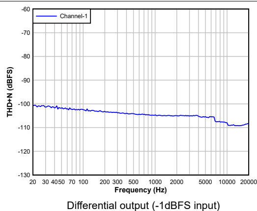
Figure 5-20. DAC THD+N Level vs Frequency
