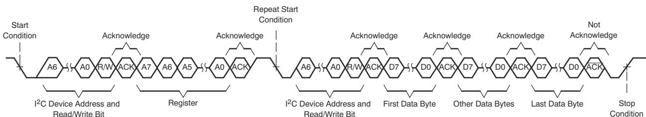
Figure 6-101. I 2 C Multiple-Byte Read Transfer
