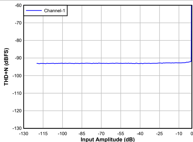
Figure 5-4. ADC THD+N Level vs Input
