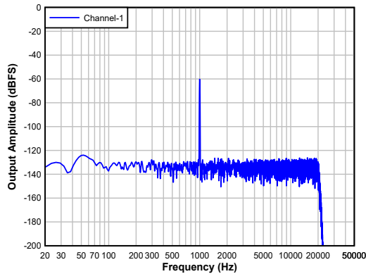
Figure 5-9. ADC Frequency Response
