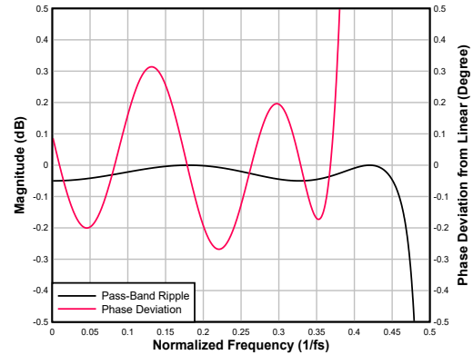
Figure 6-84. Low-latency Interpolation Filter Pass-Band Ripple and Phase Deviation
