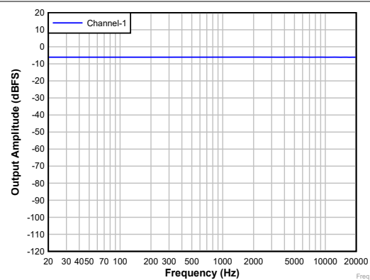
Figure 5-28. DAC Frequency Response
