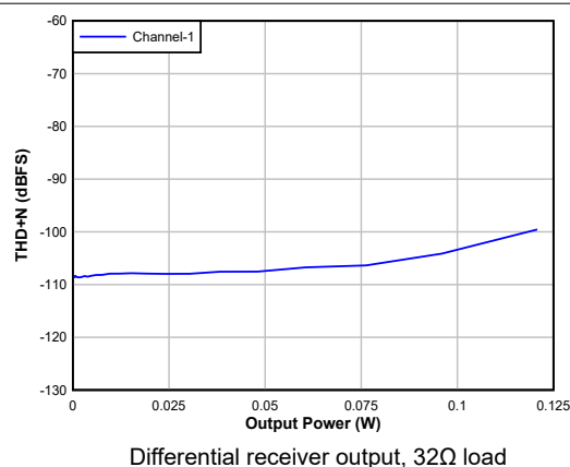
Figure 5-18. DAC THD+N Level vs Output Power
