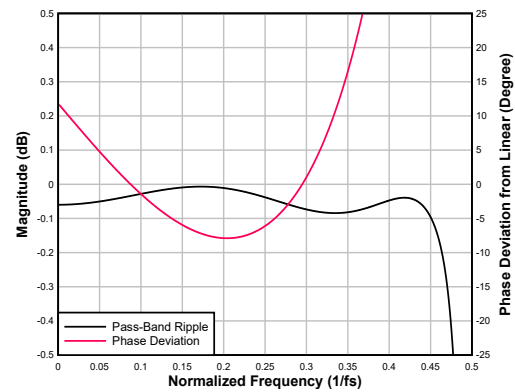
Figure 6-88. Ultra-Low-Latency interpolation Filter Pass-Band Ripple and Phase Deviation
