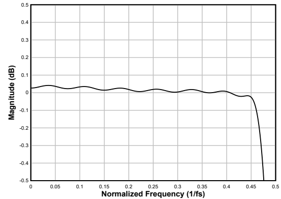
Figure 6-33. Linear-phase Decimation Filter Pass-Band Ripple
