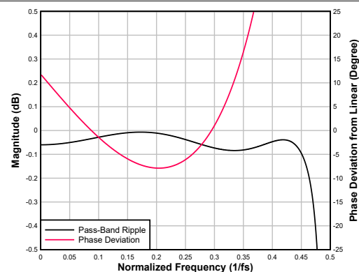
Figure 6-104. Ultra-Low-Latency interpolation Filter Pass-Band Ripple and Phase Deviation
