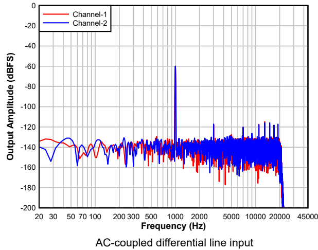
Figure 5-15. ADC FFT with -60dBFS Input
