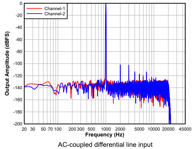
Figure 5-16. ADC FFT with -1dBFS Input
