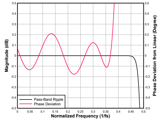
Figure 6-98. Low-latency Interpolation Filter Pass-Band Ripple and Phase Deviation
