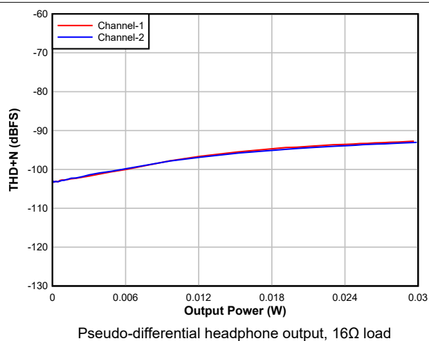
Figure 5-24. DAC THD+N Level vs output power
