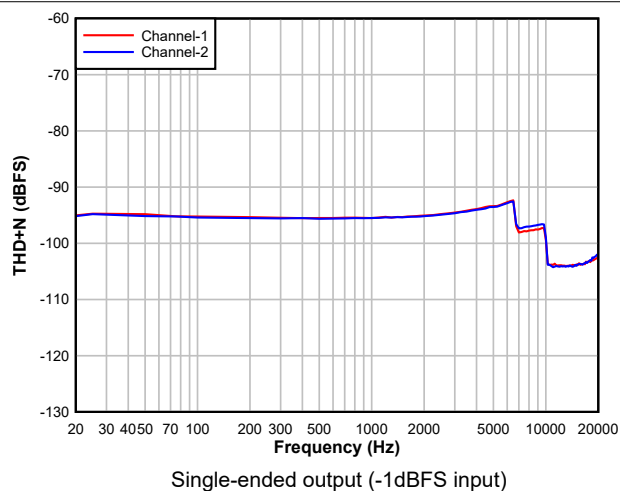
Figure 5-26. DAC THD+N Level vs Frequency
