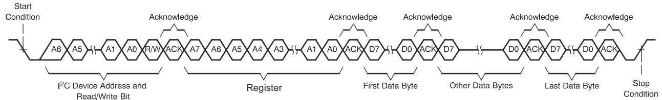
Figure 6-111. I 2 C Multiple-Byte Write Transfer
