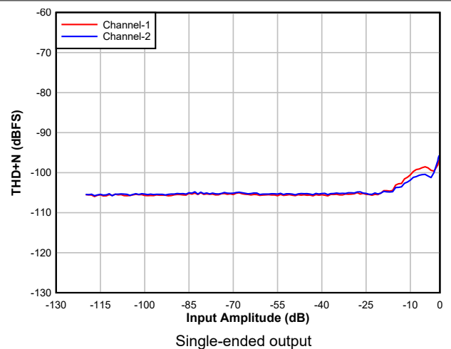
Figure 5-20. DAC THD+N Level vs Input
