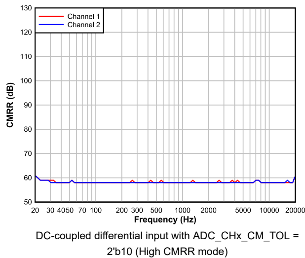
Figure 5-17. ADC CMRR vs Frequency
