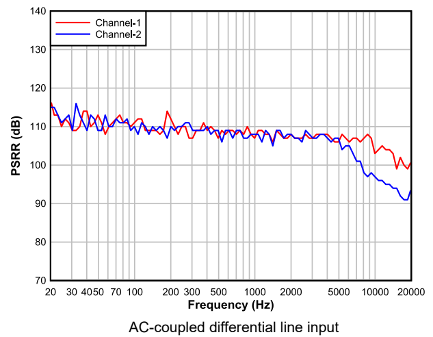
Figure 5-18. ADC PSRR vs Frequency
