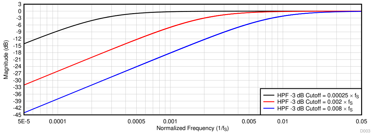
Figure 6-70. HPF Filter Frequency Response Plot
