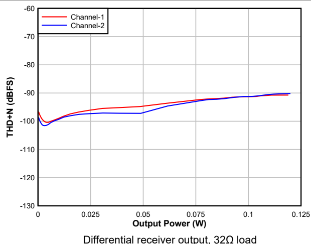
Figure 5-22. DAC THD+N Level vs output power
