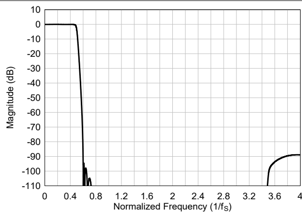
Figure 6-103. Ultra-Low-Latency interpolation Filter Magnitude Response
