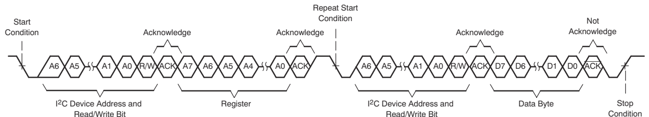
Figure 6-112. I 2 C Single-Byte Read Transfer
