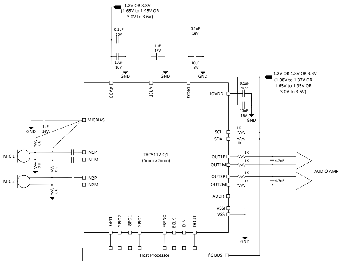
Figure 8-1. Stereo Microphone with Stereo Lineout Block Diagram
