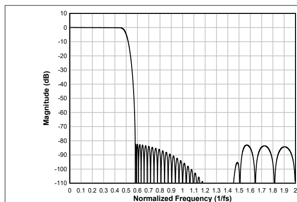
Figure 7-81. Linear-phase Interpolation Filter Magnitude Response
