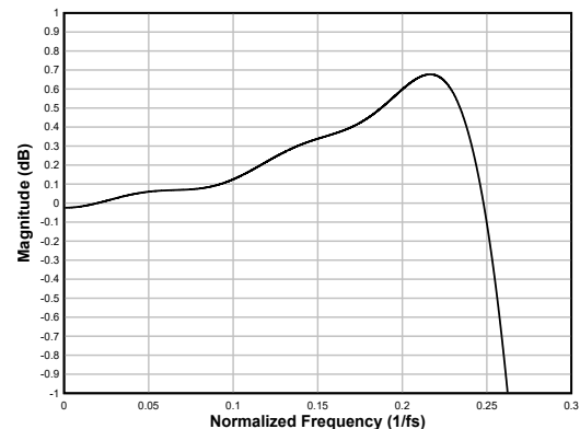
Figure 7-86. Linear-phase Interpolation Filter Pass-Band Ripple
