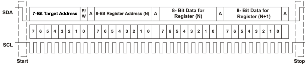
Figure 7-109. Typical I²C Sequence
