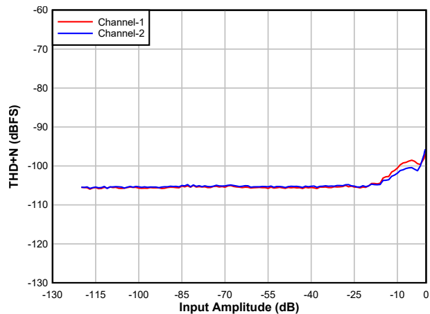
Figure 6-20. DAC THD+N Level vs Input
