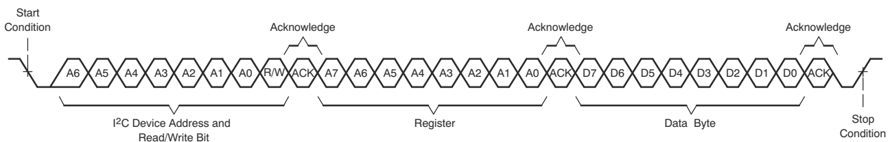
Figure 7-110. I²C Single-Byte Write Transfer
