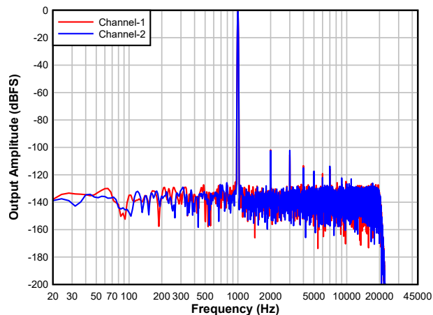
Figure 6-16. ADC FFT with -1dBFS Input
