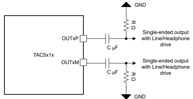
Figure 6-24. Stereo Single-ended Output Connection (OUT1x_CFG[2:0] = 3'b001)
