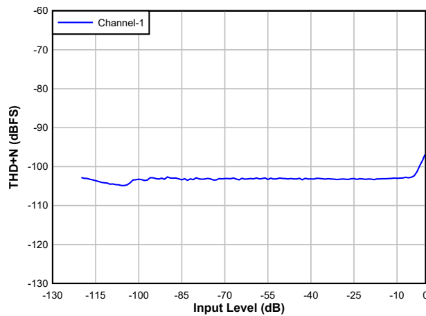
Figure 5-5. ADC THD+N Level vs Input
