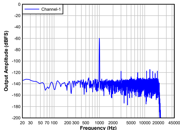
Figure 5-15. ADC FFT with -60dBFS Input
