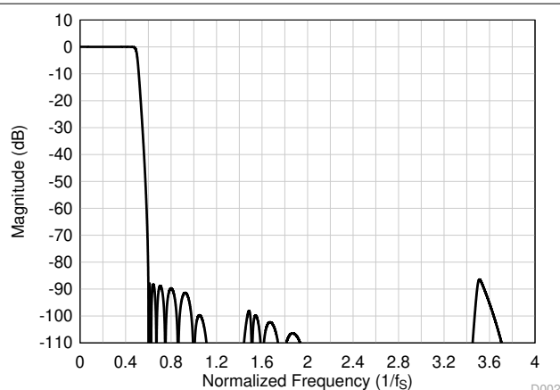
Figure 6-43. Low-Latency Decimation Filter Magnitude Response
