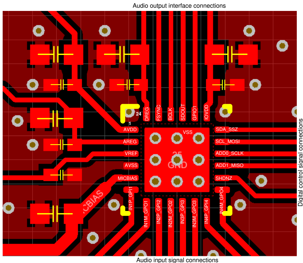
Figure 8-4. Layout Example
