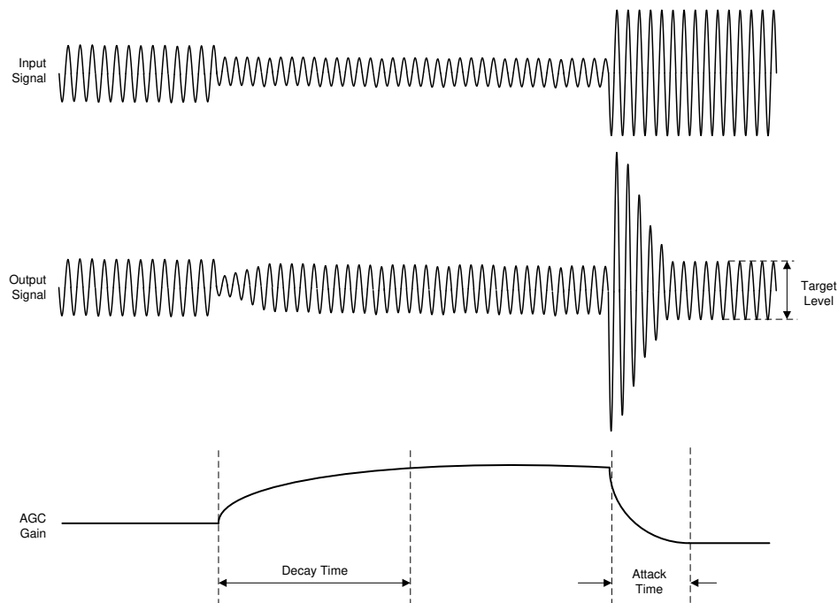
Figure 6-63. AGC Characteristics
