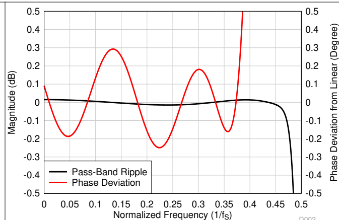
Figure 6-44. Low-Latency Decimation Filter Pass-Band Ripple and Phase Deviation
