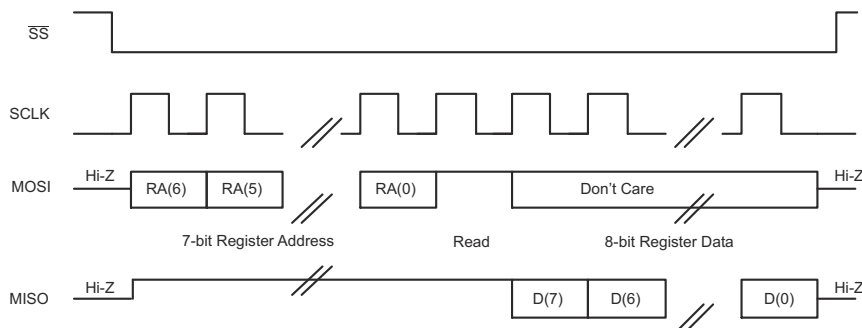
Figure 6-72. SPI Single-Byte Read Transfer
