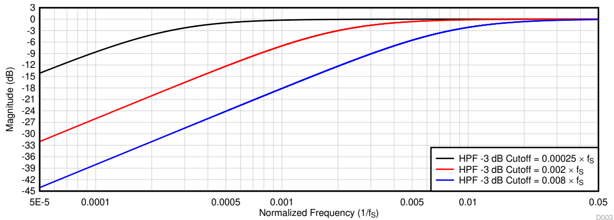
Figure 6-17. HPF Filter Frequency Response Plot
