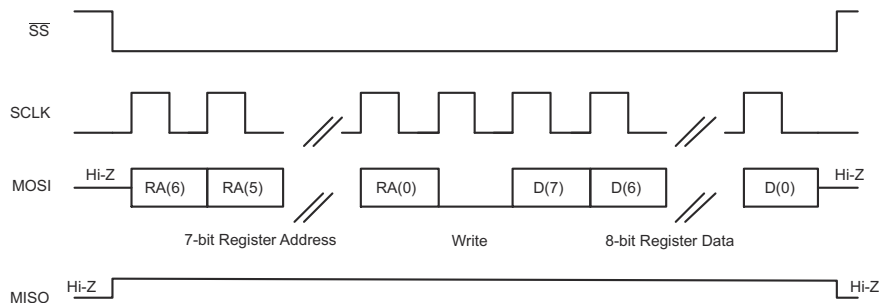
Figure 6-71. SPI Single-Byte Write Transfer
