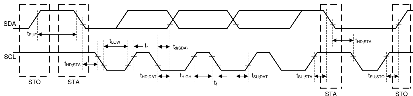
Figure 5-1. I²C Interface Timing Diagram
