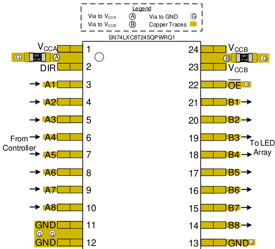
Figure 9-2. Layout Example – SN74LXC8T245PW-Q1
