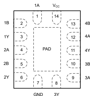
Figure 3-2. SN74LVC32A-Q1 BQA Package, 14-PIN WQFN (Top View)
