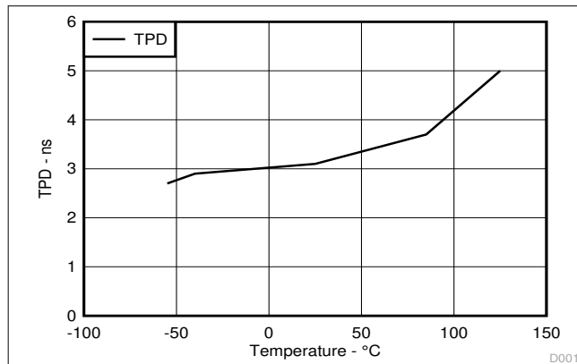
Figure 5-1. TPD Across Temperature at 3.3\text{V } V_{CC}
