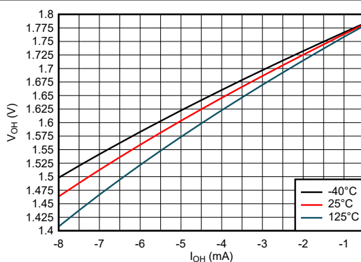
Figure 5-13. Output Voltage vs Current in HIGH State; 1.8V Supply
