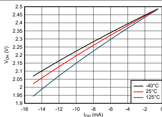
Figure 5-11. Output Voltage vs Current in HIGH State; 2.5V Supply
