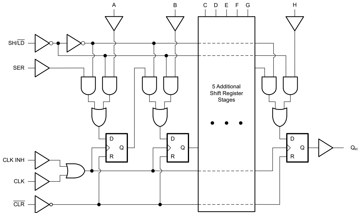
Functional Diagram
