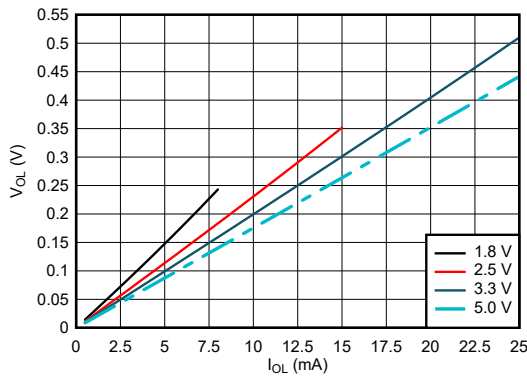
Figure 5-6. Output Voltage vs Current in LOW State
