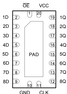
Figure 4-1. SN74LV8T574-Q1 RKS Package (Top View)
