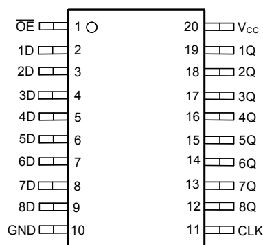
Figure 4-2. SN74LV8T574-Q1 PW, DGS Package (Top View)
