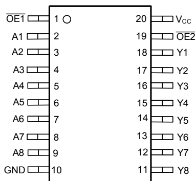
Figure 4-1. PW and DGS Package, 20-Pin TSSOP (Top View)
