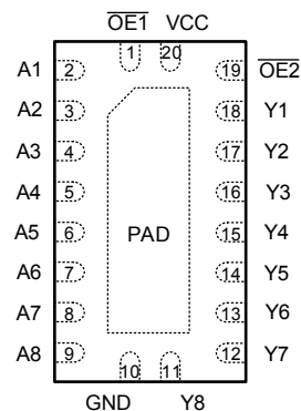
Figure 4-2. RKS Package, 20-Pin VQFN (Transparent Top View)
