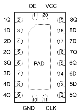
Figure 4-1. SN74LV8T374 RKS Package (Top View)
