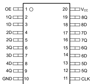
Figure 4-2. SN74LV8T374 PW, DGS Package (Top View)
